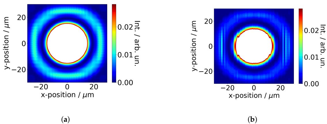
Figure 5. Simulated far-field distribution of the reflected light at 50\ \mu\text{m} distance from the surface. (a) Unstructured titanium. (b) Sinusoidally structured titanium surface (600 nm period, 300 nm height).
