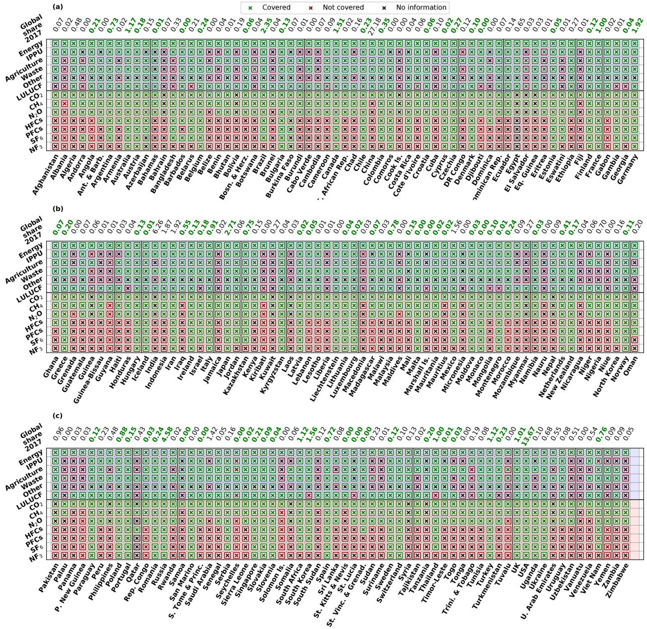
Figure A1. Sectors and Kyoto GHGs covered by NDCs on a per-country level. Crosses: ± explicitly mentioned coverage, squares: adapted coverage used in NDCmitiQ. EU target information: shown for single countries (e.g. Germany). The per-country share of global Kyoto GHG emissions is presented (for 2017, based on PRIMAP-hist v2.1 HISTCR, GWP AR4 excluding LULUCF, and bunker fuels). Shares displayed in green: target is intended to be economy-wide. NDC submissions until 17 April 2020.
