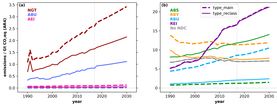
Figure 3. Aggregated time series of national baseline (non-mitigated) emissions for all countries with a certain NDC mitigation target type (for type_main and type_reclass). Emissions based on PRIMAP-hist v2.1 and downscaled SSP2 marker scenario (data source: Gütschow et al., 2019, 2020b, see Sect. 2.2). Emissions from LULUCF and bunker fuels are excluded (bunker fuels: international shipping and aviation; not attributed to individual countries under the United Nations Framework Convention on Climate Change (UNFCCC); Gütschow et al., 2021). A vertical line indicates the last year of historical data (2017). USA: classified as “No NDC”. NDC submissions until 17 April 2020.
