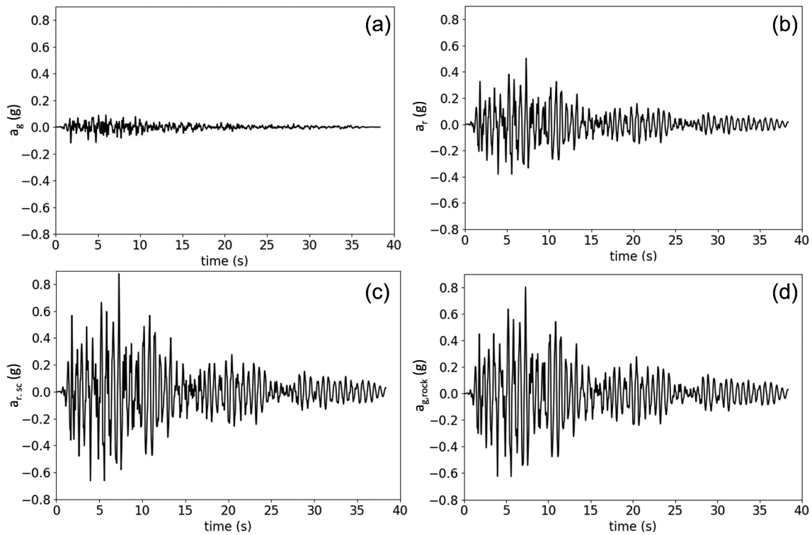
Figure 4. Procedure for filtering and scaling of the input ground motion: (a) unscaled input ground acceleration a_g , (b) filtered relative acceleration a_r at the effective modal height h_{er} , (c) scaled and filtered relative acceleration a_{r,sc} at the mechanism height h_m and (d) final input signal at base of rocking mechanism a_{g,rock} .
