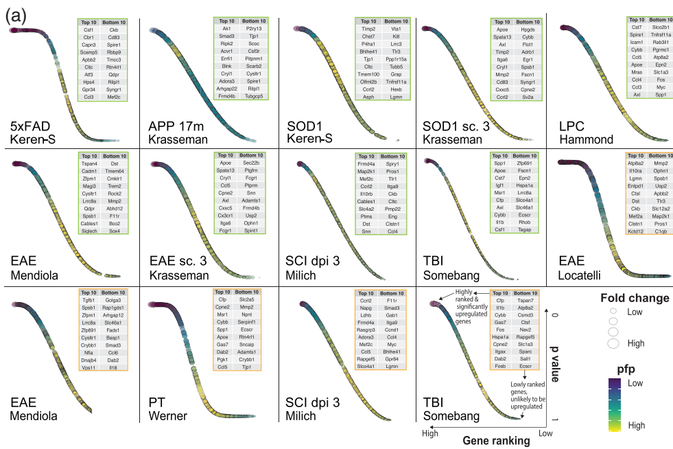
FIGURE 2 Clustering analysis connects the transcriptomic responses adopted by microglia and MCs in disease. (a) Bubble plots showing gene ranking using Common Gene set A by order of upregulation (x-axis) with associated p -values (y-axis), fold-change (bubble size) and percentage of false predictions (pfp) values (bubble color) for selected MC (the cell type indicated by orange boxes) and microglia (indicated by green boxes) populations. The top- and bottom-ranked genes are listed in these boxes, placed at the top right of each plot, for MC (orange boxes) and microglia (green boxes) populations. (b–e) UMAP plots of 18 microglia and 12 MCs samples pseudocolored by cell type (b), disease (c), sequencing technology (d) or study (e). UMAPs were run on gene rank values for the 319 genes of Common Gene set A. See also Table S2 for a list of populations used with their study and disease origins. (f) Heatmap showing gene rank values for the 319 genes of Common Gene set A in order of upregulation for MC and microglial populations. Clustering was performed on both rows (genes) and columns (populations). See also Table S2 for a list of populations used with their study and disease origins in order of the clustering arrangement shown in the heatmap
