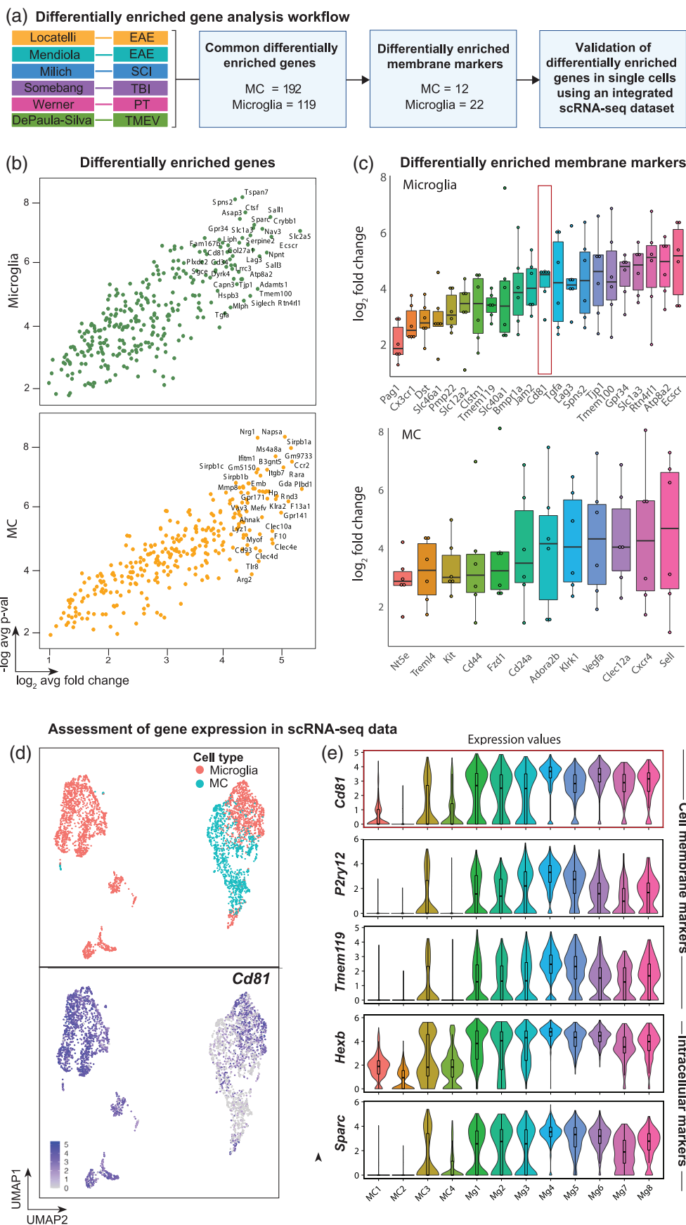
FIGURE 7 Cross-disease analysis reveals Cd81 as a microglial-enriched gene in neuroinflammation. (a) Flow chart analysis pipeline used to identify differentially enriched microglial and MC genes in the inflamed brain. Six studies that simultaneously analyzed microglia and MCs in the CNS were used to identify 192 and 119 differentially enriched ( p > .05 , \log_2 > 1 ) MC and microglia genes, respectively. This gene list was filtered in Uniprot to identify membrane expressed genes, which were subsequently validated with expression data using an integrated scRNA dataset. (b) Volcano plots showing all genes differentially enriched by microglia and MCs in EAE, SCI, TBI, PT and TMEV. The top 35 differentially enriched genes are annotated. See also Table S6 for a list of these genes. (c) Box plots showing differentially enriched surface/plasma membrane-expressed genes for microglia and MCs. (d) UMAPs showing single-cell gene expression overlays for Cd81 in MC and microglial clusters identified in the integrated scRNA-seq dataset. (e) Violin plots showing the expression of Cd81 relative to nominal microglia-specific genes in the 12 myeloid clusters
