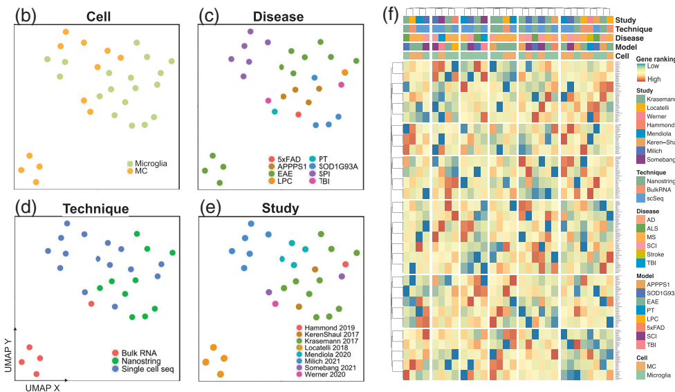
FIGURE 2 Clustering analysis connects the transcriptomic responses adopted by microglia and MCs in disease. (a) Bubble plots showing gene ranking using Common Gene set A by order of upregulation (x-axis) with associated p -values (y-axis), fold-change (bubble size) and percentage of false predictions (pfp) values (bubble color) for selected MC (the cell type indicated by orange boxes) and microglia (indicated by green boxes) populations. The top- and bottom-ranked genes are listed in these boxes, placed at the top right of each plot, for MC (orange boxes) and microglia (green boxes) populations. (b–e) UMAP plots of 18 microglia and 12 MCs samples pseudocolored by cell type (b), disease (c), sequencing technology (d) or study (e). UMAPs were run on gene rank values for the 319 genes of Common Gene set A. See also Table S2 for a list of populations used with their study and disease origins. (f) Heatmap showing gene rank values for the 319 genes of Common Gene set A in order of upregulation for MC and microglial populations. Clustering was performed on both rows (genes) and columns (populations). See also Table S2 for a list of populations used with their study and disease origins in order of the clustering arrangement shown in the heatmap
