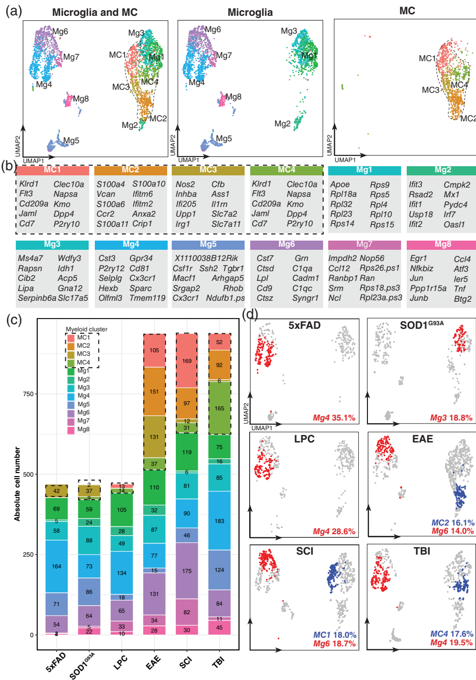
FIGURE 5 Integrative analysis of single-cell RNA-sequencing datasets identifies conserved and disease-specific MC and microglial clusters across six disease models. (a) UMAPs of myeloid cells from the downsampled LIGER-integrated dataset overlaid by either microglia (2814 cells) and/or MC clusters (1407 cells). See also Figure S1 for the expression of cell type-specific genes used to annotate cell types. (b) Top 10 differentially expressed genes per cluster. Differentially expressed genes were defined as genes enriched in a cluster versus all other clusters ( \log_2 fold-change >0.25 , p value <.01 ) by Wilcoxon rank sum test. (c) Absolute cell numbers of microglial and MC clusters across the six disease models. Datasets were downsampled prior to integration to ensure equal representation across disease models (469 microglia from each six disease models, 469 MCs from EAE, TBI, and SCI). Absolute cell numbers for each disease model prior to downsampling were 685 MCs and 1960 microglia in LPC-induced demyelination; 3234 MCs and 1468 microglia in EAE; 182 MCs and 3620 microglia in 5xFAD; and 72 MCs and 1136 microglia in SOD1 G93A , 14,243 MCs and 17,739 microglia in SCI; and 612 MCs and 8434 microglia in TBI. (d) Highest proportional representation of MC (blue) and microglia (red) clusters for each disease model overlaid onto UMAPs of myeloid cells from each disease model. Numbers represent the relative percentage of each of the myeloid clusters of the total myeloid pool in each disease model. Disease models 5xFAD, SOD1 G93A , and LPC-induced demyelination contain only microglia (469 cells per disease model), whereas EAE, TBI and SCI contain both microglia and MCs (938 cells per disease model)
