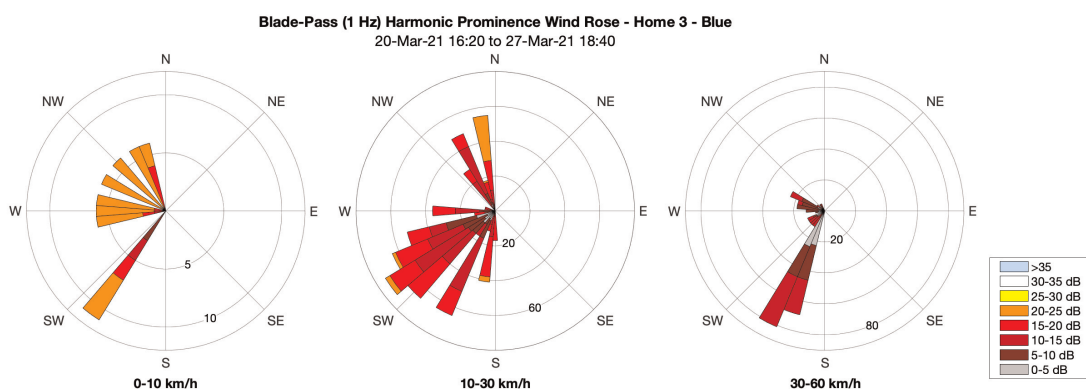
Figure 15. Harmonic prominence wind roses for three wind-speed ranges for Home 3. The strongest H_p is at the lowest windspeed and this is most consistently dominant when the wind is from the west through to northwest. That is, the sectors of the wind rose in these directions are almost entirely made up of 10-minute intervals where the H_p was between 20 and 25 dB (orange). By comparison, where the wind was from the southwest, only about 1/3 of the sound files have this level. At the highest windspeeds, no instances of even 15–20 dB H_p can be seen.
