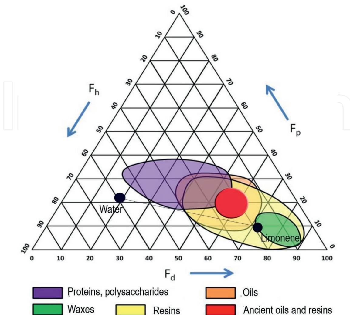
Figure 4. Masschelein–Kleiner diagram: Solubility of natural film-forming substances and position in the triangle of the two main components of the proposed cleaning formulas: water and limonene. Note how there is partial overlap between resins and oily layers.
