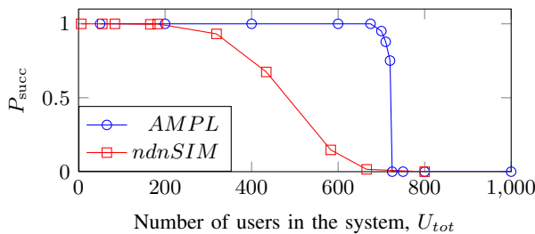
Fig. 5. Success probability, P_{succ} , in content retrieval evaluated using the proposed optimal content placement and ndnSIM with the LRU caching policy varying the number of users in the system.
