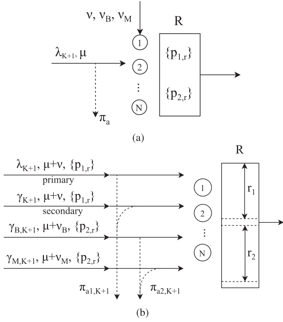
Fig. 2. Original and equivalent ReLS models for node K + 1 . (a) Original system with events. (b) Equivalent system with additional arrival flows.
