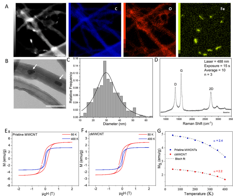
Fig. 1. Physicochemical characterization of cMWCNT. (A) EDS mapping: Carbon (marked as C), oxygen (marked as O) and iron (marked as Fe) (Scale bar 50 nm). (B) TEM images of cMWCNT, white arrow: Fe nanoparticles encapsulated in the cMWCNT (Scale bar 50 nm). (C) Diameter distribution for cMWCNT measured from series of TEM images. (D) Raman spectrum of cMWCNT. (E-F) Magnetic field dependence of magnetization plotted at 50 K and 400 K for (E) pristine MWCNTs and (F) cMWCNT. Saturation magnetization (G) versus temperature for pristine MWCNT and cMWCNT.
