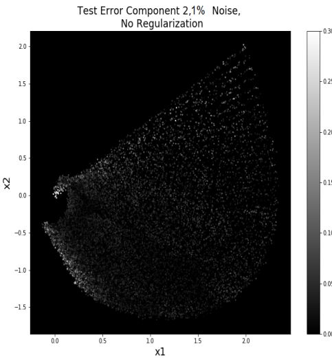
(c) Test error non-regularized network, 1% noise in the data, second component.
