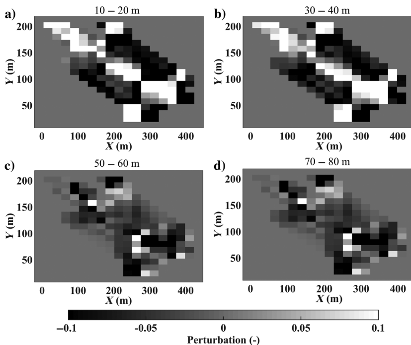
Figure 18. The checkerboard test performed to the hypothetical geometry of acquisition in Figure 17. The horizontal sections showing the layers at depths of (a) 10–20 m, (b) 30–40 m, (c) 50–60 m, and (d) 70–80 m.
