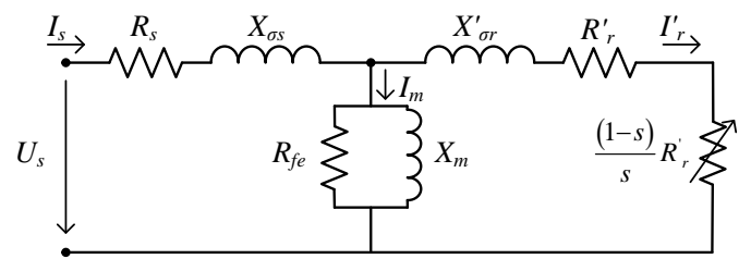
Fig. 2. Single-phase equivalent circuit.
