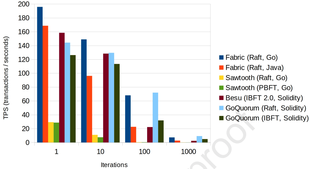
Figure 6: Iteration test: TPS for different read/write amounts. A pair of read/write operations (iteration = 1) represents an update on a single asset. A set of multiple read/write operations represents a transaction updating multiple assets.
