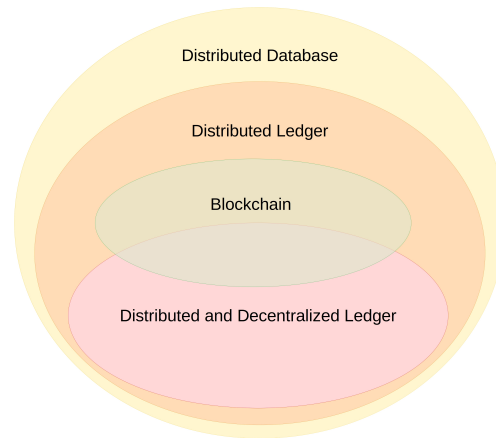
Figure 1: The relationships among the distributed database, distributed ledger (DLT), and blockchain technologies. In particular, a DLT is a distributed database, structured as a ledger. A DLT can be decentralized or not, depending on its governance model. A blockchain is a DLT that uses a list of blocks to represent the ledger. Each block contains the hash of the header of its predecessor. Blockchain technology is associated with many interesting properties, such as immutability; however, such properties only characterize decentralized blockchains [14].
