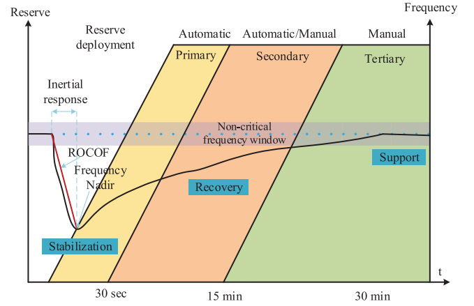
FIGURE 2 Frequency response stages defined by the ENTSO-E
