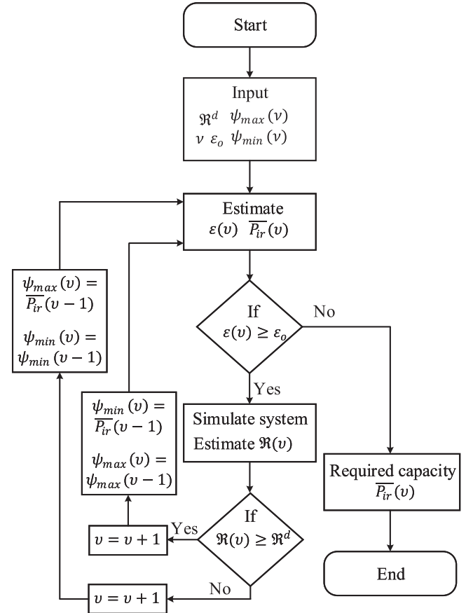
FIGURE 5 Flowchart of region reduction iterative algorithm (RRIA)
