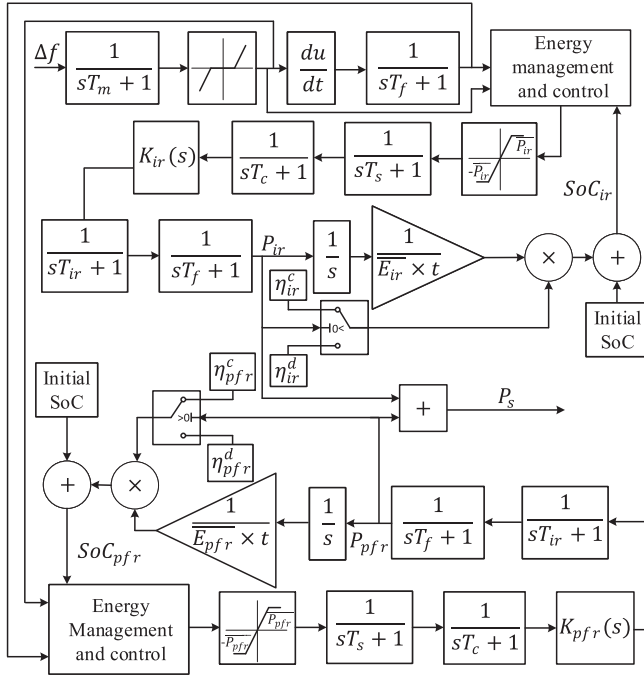
FIGURE 4 Frequency response model of HESS
