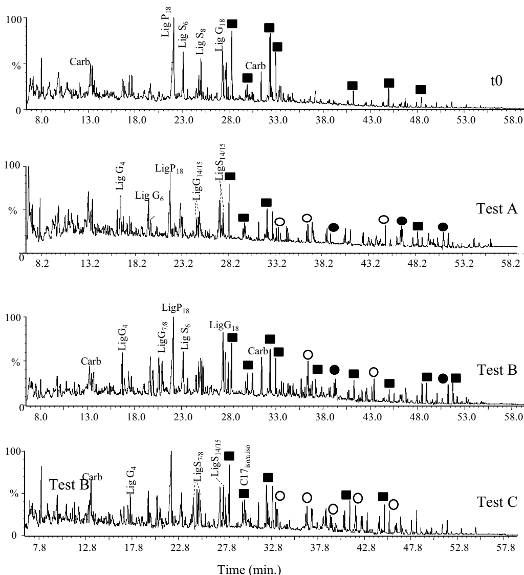
Fig. 2 Total ion chromatograms of thermochemolysis products released from initial and final compost samples Lig lignin, filled square fatty acids, filled circle alkyl-dioic acids, circle hydroxy acids
