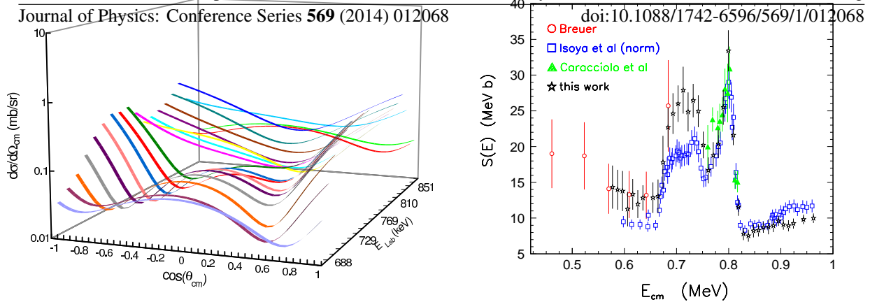
Figure 2. (Left panel) Best fits of ^{19}\text{F}(p,\alpha_0) experimental angular distributions in terms of Legendre polynomials, as a function of the bombarding energy. (Right panel) ^{19}\text{F}(p,\alpha_0) S -factor extracted in the present experiment [11] and compared with literature data [21, 27, 28] as reported in NACRE [26].
