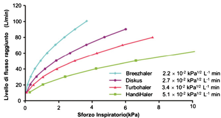
Figure 3 Resistance to air flow recorded with the main devices.
