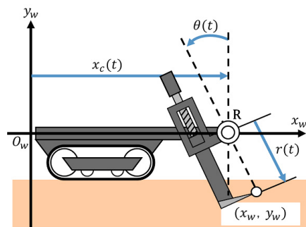
Fig. 7. Coordinates and variables for the harvester
