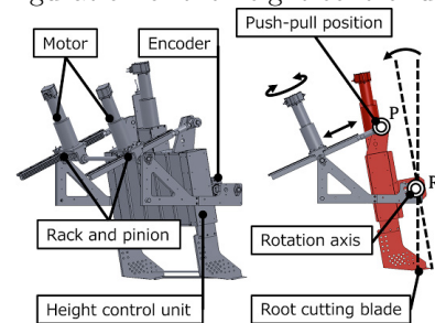
Fig. 4. Configuration of the angle control unit
