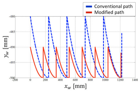
Fig. 13. Comparison of path of (x_w, y_w)
