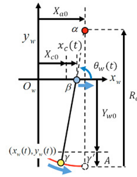
Fig. 11. Coordinate and variables for transition motion in Path 1
