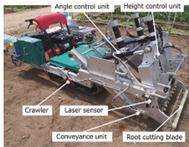
Fig. 1. Developed automatic spinach harvester
