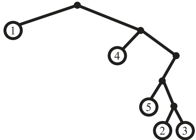
Fig. 1 An optimal binary tree for instance I = ((1, 4), (2, 1), (2, 2), (2, 3), (4, 5)) . The numbers on vertices identify leaves. Solid black points are non-leaf vertices. The objective value is 0 + 0 + 2 + 3 + 0 = 5 .
