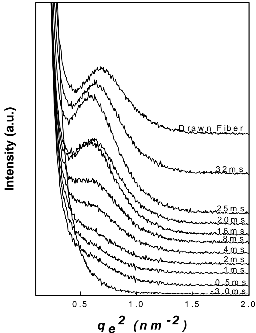
Fig. 13. The SAXS x-ray intensity profile for PTT fibers: The elapsed times were noted inside the figure frame
