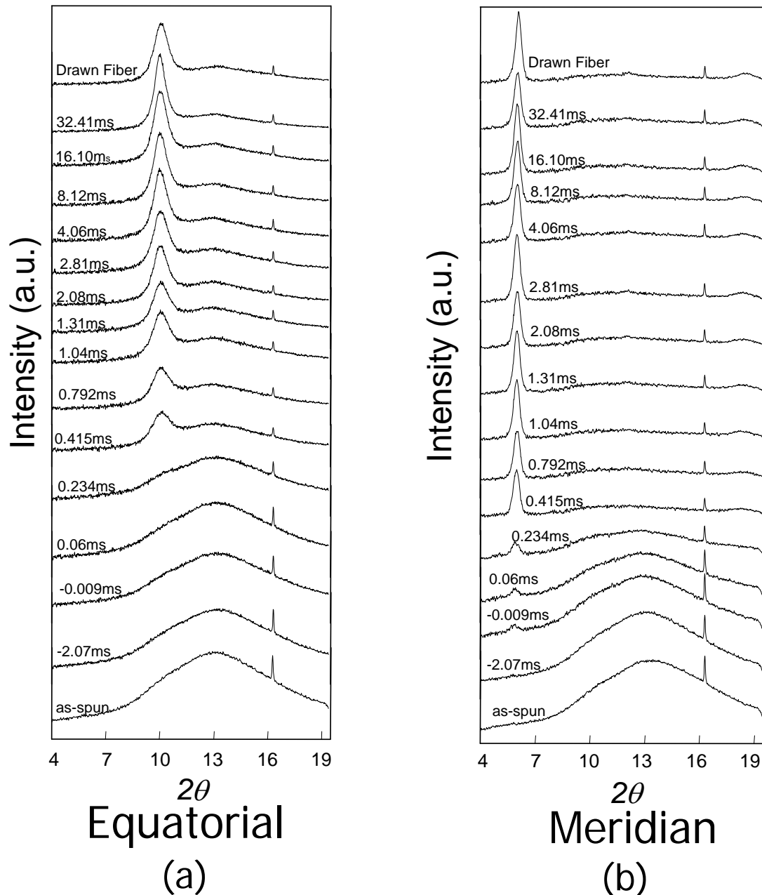
Fig. 5. The X-ray intensity profile for PTT fibers: (a) equatorial direction (b) meridional direction The elapsed times were noted inside the figure frame
