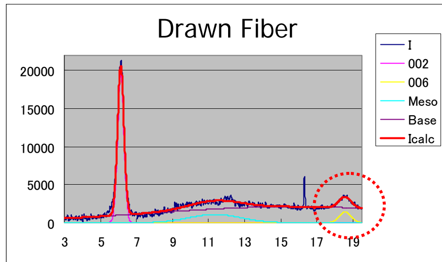
Fig. 7. Meridional intensity profiles including peak separation result.
