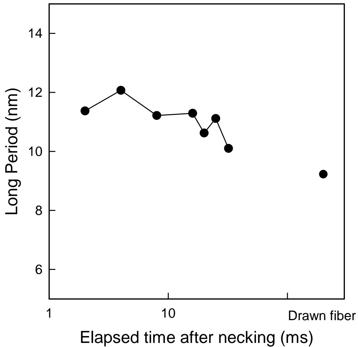
Fig. 14. Long Period obtained from SAXS image.
