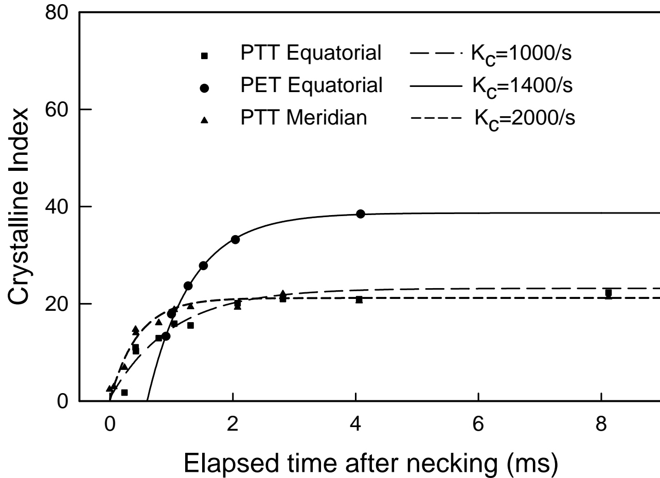
Fig. 8. Changes of the crystallinity indices in the equatorial and meridional directions for PTT fibers with elapsed time. The crystallinity index for PET fiber was plotted. The crystallization rates ( K_C ) were indicated in legend.
