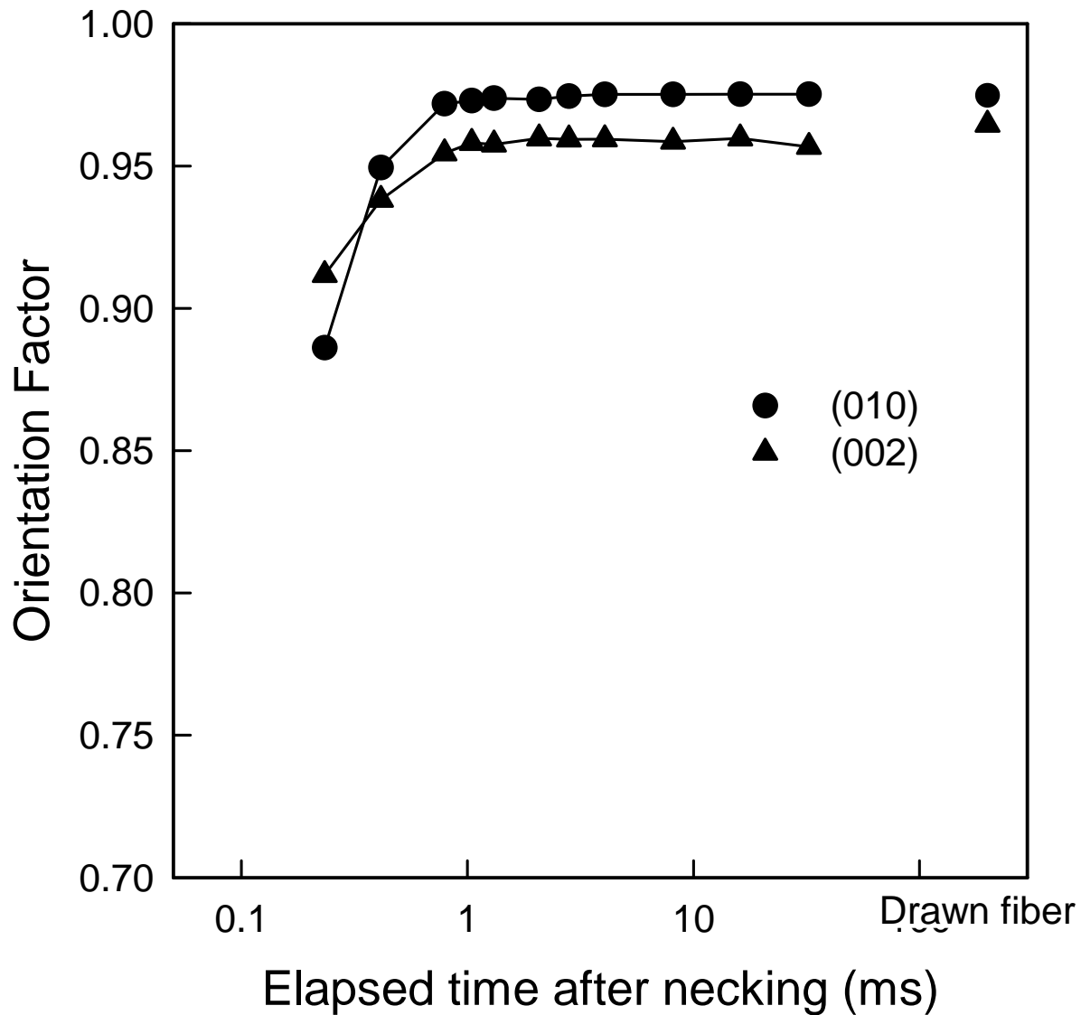
Fig. 11. Crystal orientation factor calculated from (010) (a) and (002) (b) diffractions for PTT fibers.
