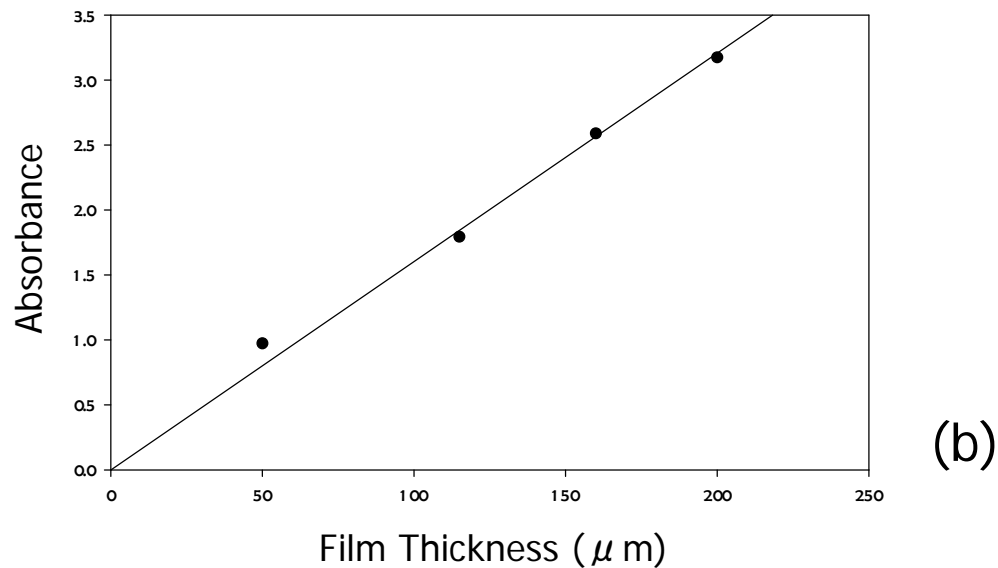
Fig. 1. (a) FT-IR Spectra of PTT films with various thicknesses. (b) IR absorbance at 943\text{cm}^{-1} as a function of film thickness.
