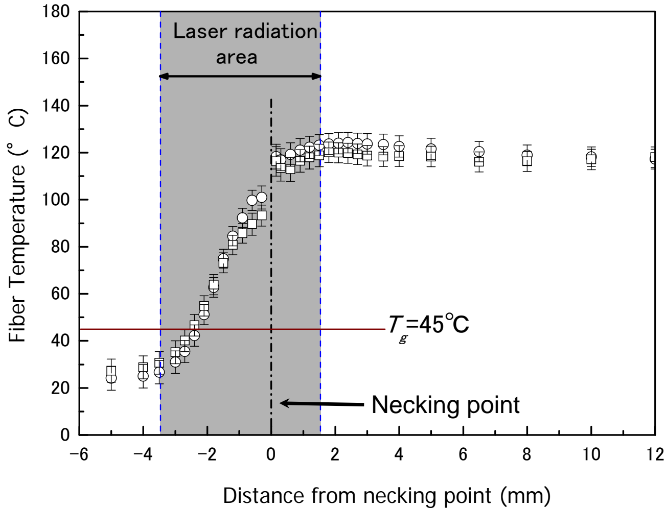
Fig. 3. Fiber Temperature profiles along the before and after necking with distance from the laser axis for PTT fiber. Fiber temperature was measured twice to get accuracy.
