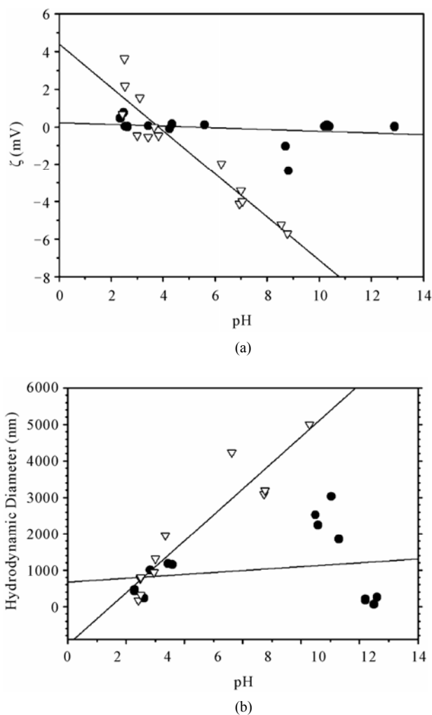
Figure 3. Zeta-potential (a) and particle size (b) of pure (●) and insulin-loaded (▽) PEG-POSS nanoparticles with respect to the pH.
