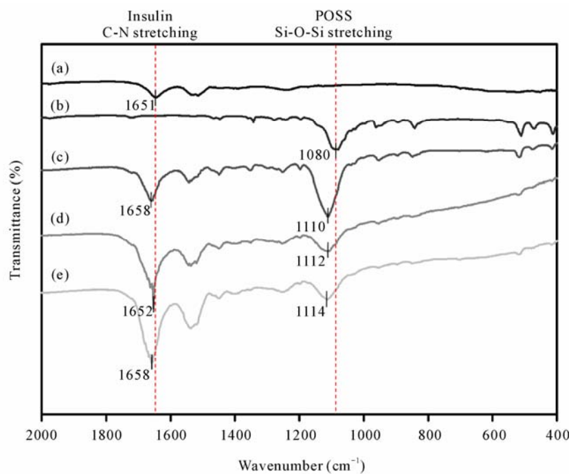
Figure 2. FTIR spectra of (a) pristine insulin, (b) pure PEG-POSS nanoparticles, and insulin-loaded PEG-POSS nanoparticles with different amount of insulin of (c) 0.5, (d) 0.9 and (e) 1.3 mg.
