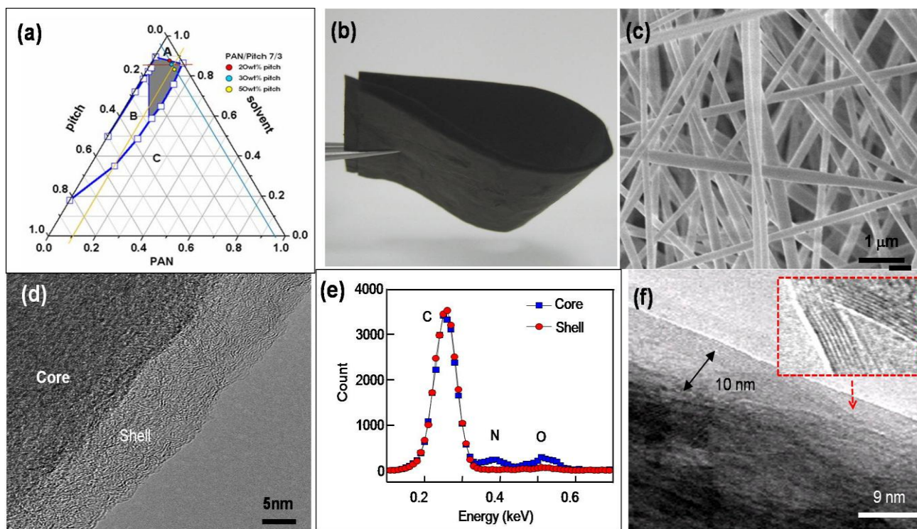
Fig. 1. (a) PAN–pitch–solvent ternary phase diagram (b) Photograph showing a bendable CNFs (c) SEM image of CNFs (d)TEM image of CNFs (e) EDX spectroscopy of air-stabilized nanofibers (f) TEM of a CNFs thermally treated up to 2800°C in argon.
