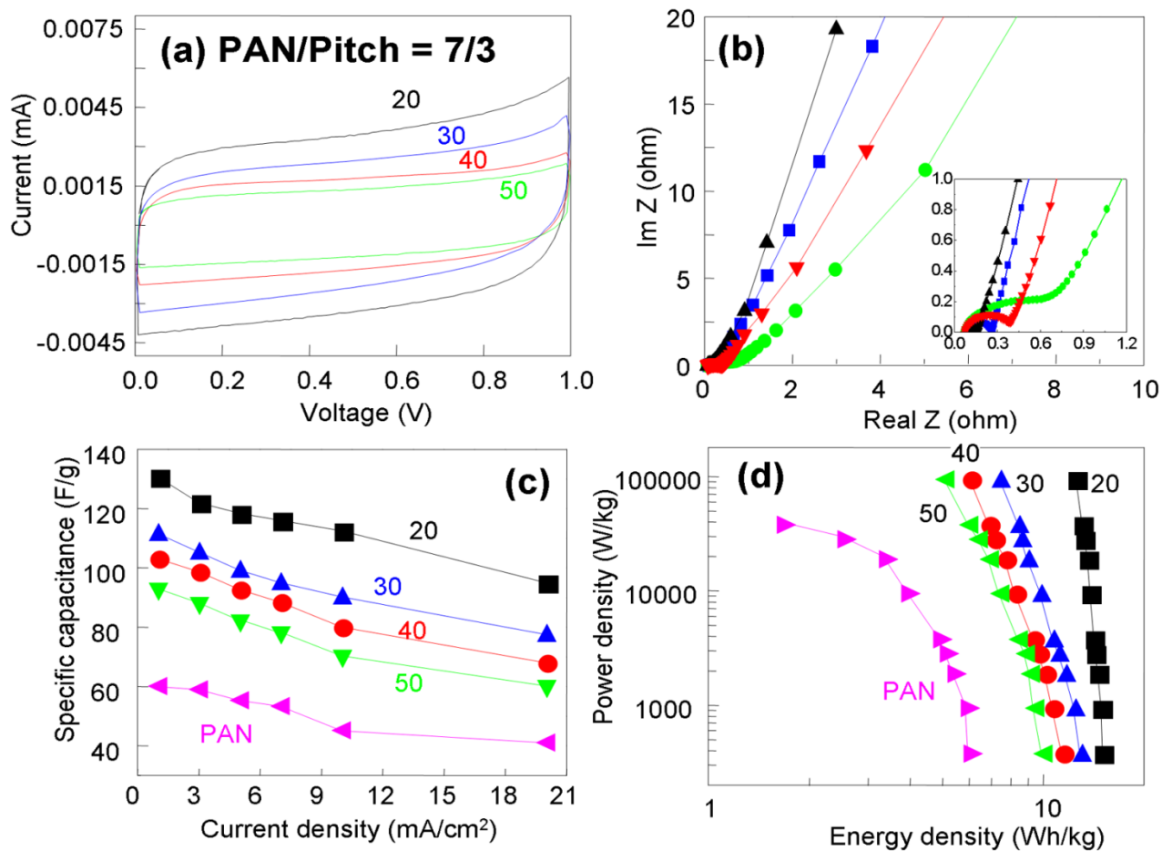
Fig. 5. (a) CVs in the range of 0-1.0 V obtained using a scan rate of 25 mVs -1 (b) Complex-plane impedance plots (c) Specific capacitances as a function of current density. (d) Ragone plots. (Note that value indicates the pitch concentration dissolved in THF.)
