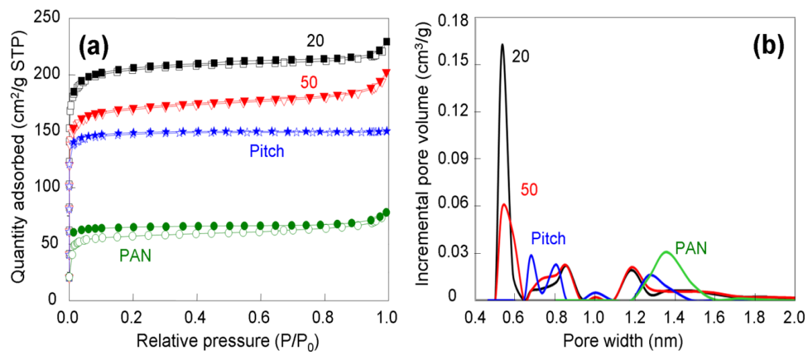
Fig. 3. (a) Nitrogen adsorption isotherms of the pure PAN- and the PAN/pitch-derived CNFs as a function of pitch concentration in THF, (b) Pore size distribution calculated by the DFT method. Note that the blend ratio of PAN/pitch is constant at 7/3.
