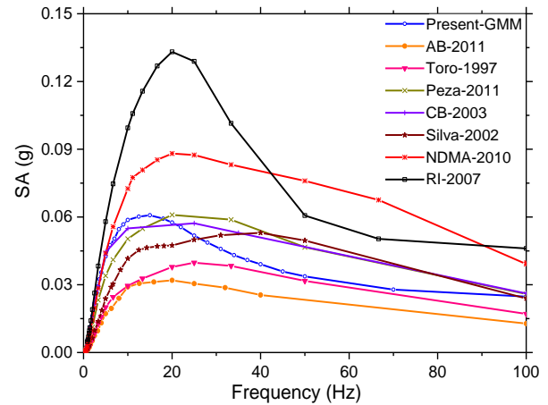
(b) 5% damped response spectra for M_w 5.0 and R_h = 50 km
