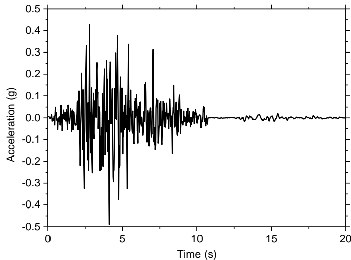
Fig. 8 Accelerogram of Koyna earthquake
