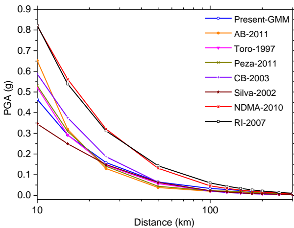
(a) PGA of M_w 6.0
