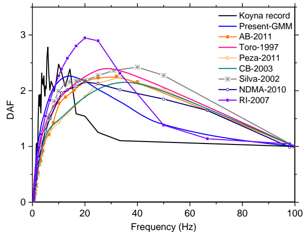
Fig. 10 Comparison of the frequency content of the Koyna earthquake with other hard-rock ground motion relations and present-GMM
