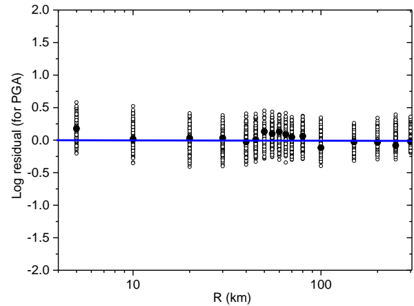
Fig. 4 Plot of residuals for M_w 7.0
