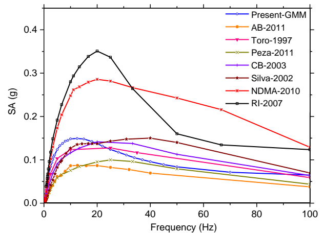
(b) 5% damped response spectra for M_w 6.0 and R_h = 50 km
