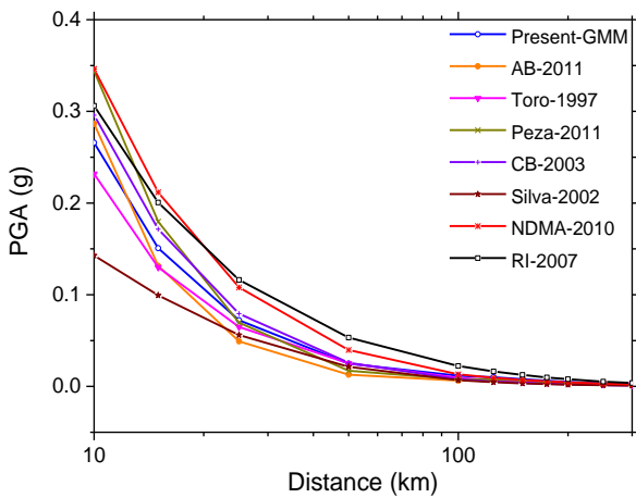
(a) PGA of M_w 5.0
