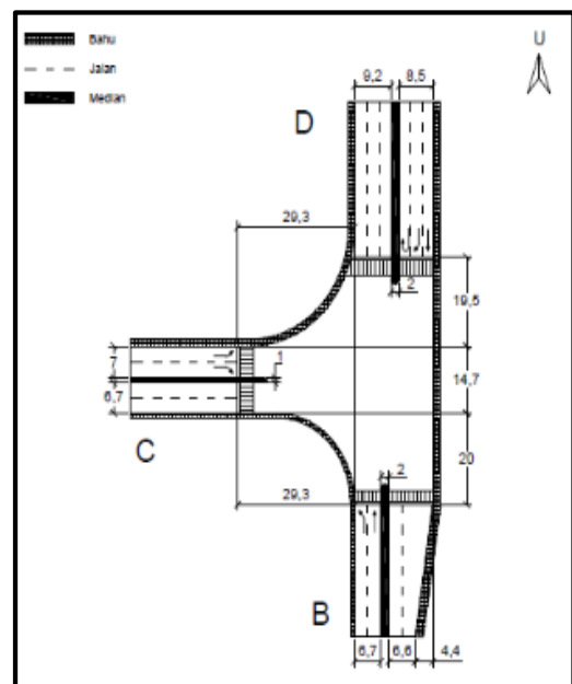
Gambar 3. Sketsa Geometrik Simpang
