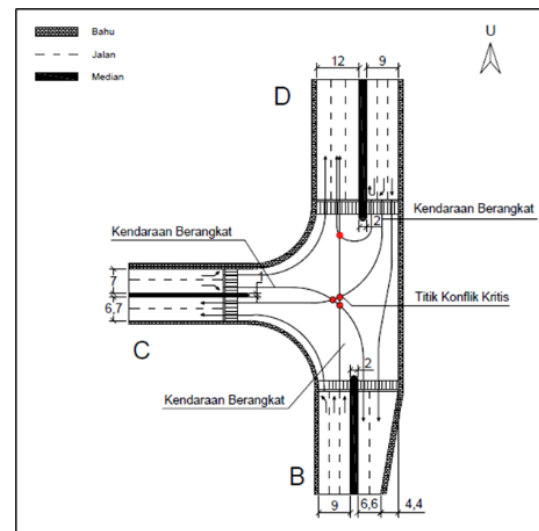
Gambar 6 Sketsa Geometrik Simpang
