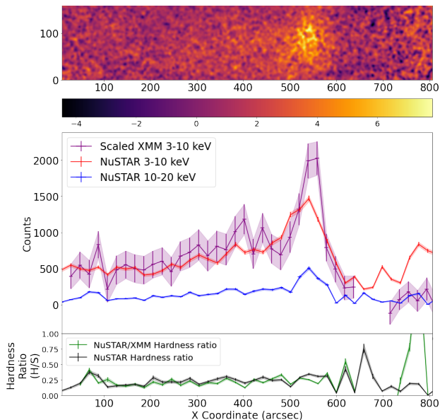
Figure 5. The scaled XMM-Newton and NuSTAR profiles around the ‘Head’ region (top) and the hardness ratio (bottom) which diverge from each other towards SS 433 (to the right of the ‘Head’ region), where we expect the greatest contribution from ghost rays.
