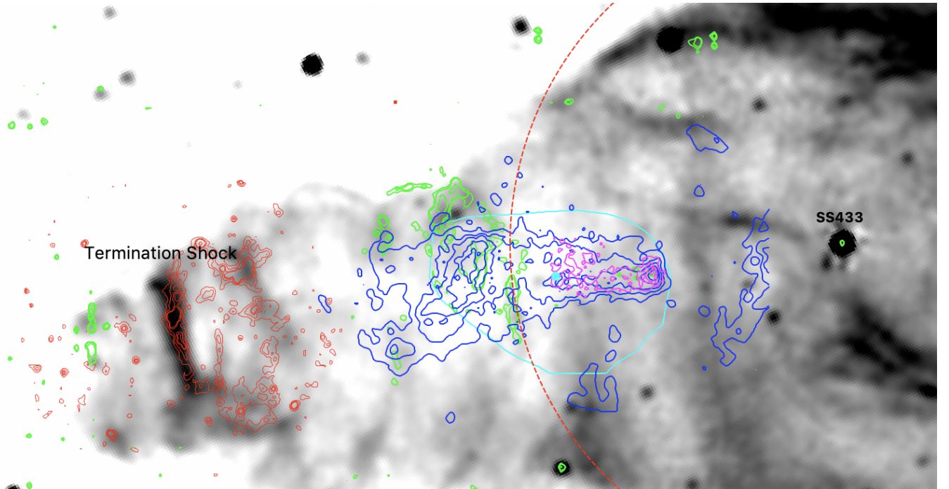
Figure 8. Multi-wavelength image of the eastern lobe of W50 bounded by SS 433 to the right and the radio ‘ear’ to the left. The radio 1.4 GHz image (Dubner et al. 1998) is shown with X-ray, optical (Boumis et al. 2007) and the HAWC emission (Abeysekara et al. 2018). Contours shown are XMM-Newton contours of the inner eastern jet covering regions e1–e2 (blue), NuSTAR coverage of the innermost region jet covering e1 (purple), XMM-Newton contours of the e3-ring region (red) overlapping the radio ‘ear’ (or termination shock), optical filaments (green) and the HAWC 4\sigma contour (cyan). We note that the blue contour running in the north-south direction in between SS 433 and the head-e1 region delineates the edge of the XMM-Newton field of view. The dashed radio circle denotes the extent of the radio shell seen to the north and south. The inner X-ray lobe is sitting within a radio ‘hole’ (or depression in radio emission), while the optical filaments partially overlap with the projection of the radio shell along the SS 433 jet axis.
