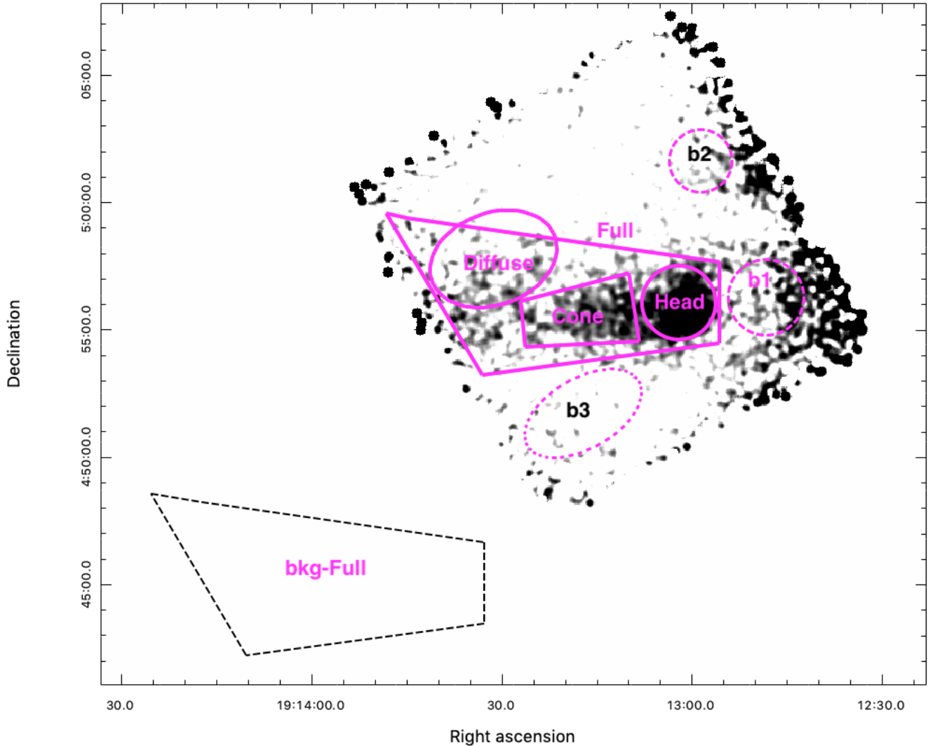
Figure A1. NuSTAR 3–10 keV image showing the background regions selected for our background analysis detailed in §A.1. The solid purple regions are the source regions selected for our main spectral analysis, while the dashed regions represent the background regions (b1, b2, b3) explored for optimizing the background selection. For the ‘Full’ source region, we chose a background from our off-source observation (dashed black polygon) with a similar PA. The final background regions selected for each of the source regions are shown in Figure 2.
