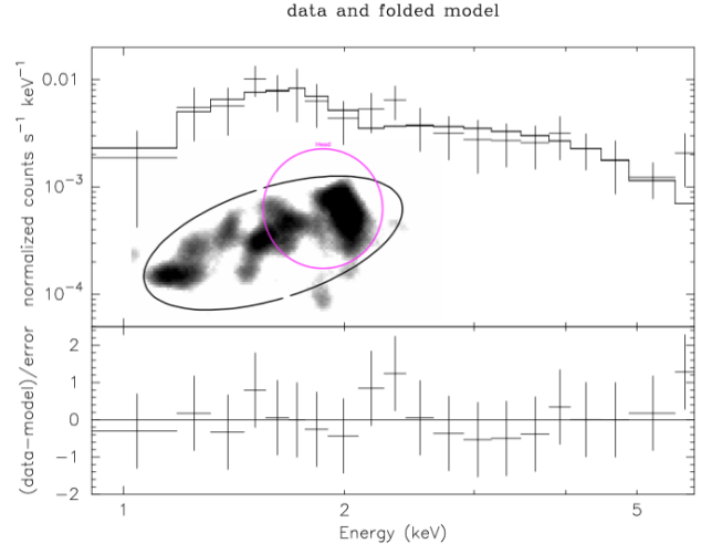
Figure 6. Chandra image (Inset) and spectrum of the inner eastern lobe overlapping with the ‘Head’ region (purple circle overlaid on the image). The image is shown on a linear scale (from 0.5 to 5 counts per pixel) and is smoothed with a Gaussian with \sigma of 7 pixels. The overlaid black ellipse shows the region used for extraction of the Chandra ACIS spectrum fitted with an absorbed power-law model with a photon index \Gamma \sim 1.5 (see §3.2.2).
