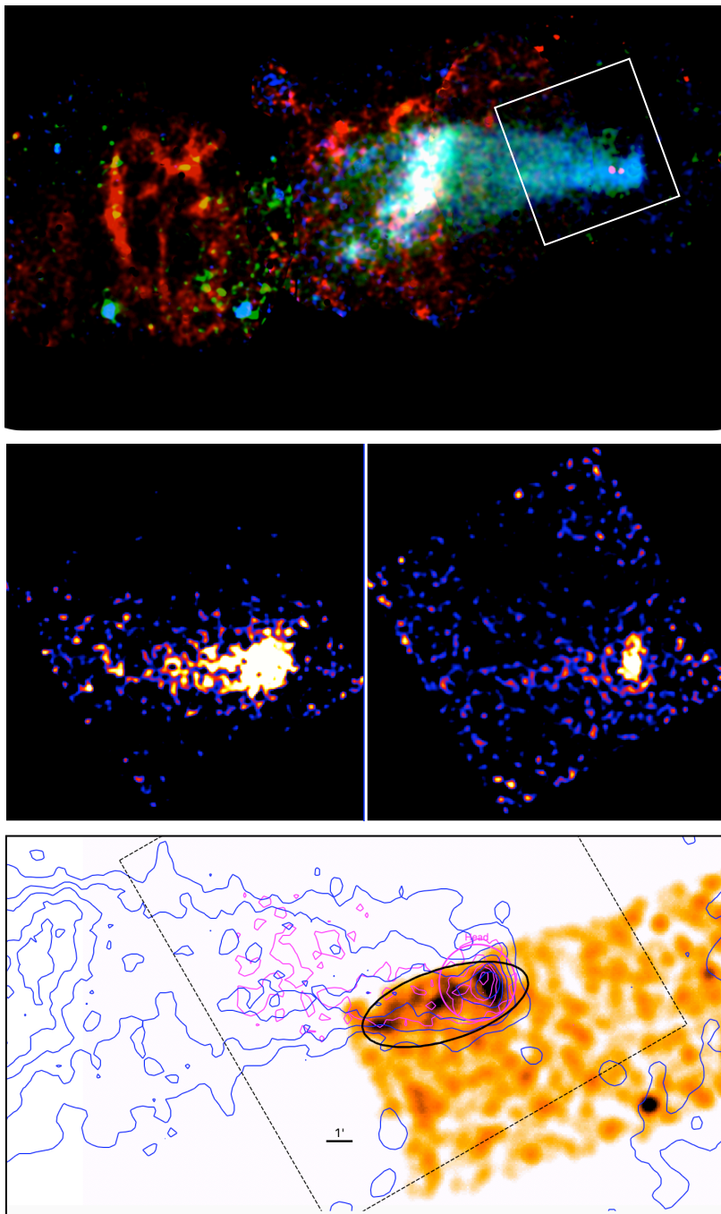
Figure 3. Top panel: An energy sliced mosaic image of W50 generated by merging exposure-corrected and smoothed new and archival XMM-Newton data. The color scheme correspond to the 0.5–1.0 keV (red), 1.0–2.0 keV (green), and 2–10 keV (blue). The white box outlines the NuSTAR FoV shown in the next panel (containing region ‘e1’). Middle panel: Combined NuSTAR FPMA and FPMB smoothed images in the 3–10 keV (left) and 10–20 keV (right) band, exposure and vignetting corrected. Bottom panel: Serendipitous partial Chandra coverage of the inner part of the eastern lobe. Contours are NuSTAR (magenta) and XMM-Newton (blue). The dashed box is the NuSTAR FoV and the ellipse (black) shows the Chandra spectral extraction region that partially overlaps the ‘Head’ region. The image is bounded by SS 433 on the right (west) and the ‘lenticular’ region on the left (east).
