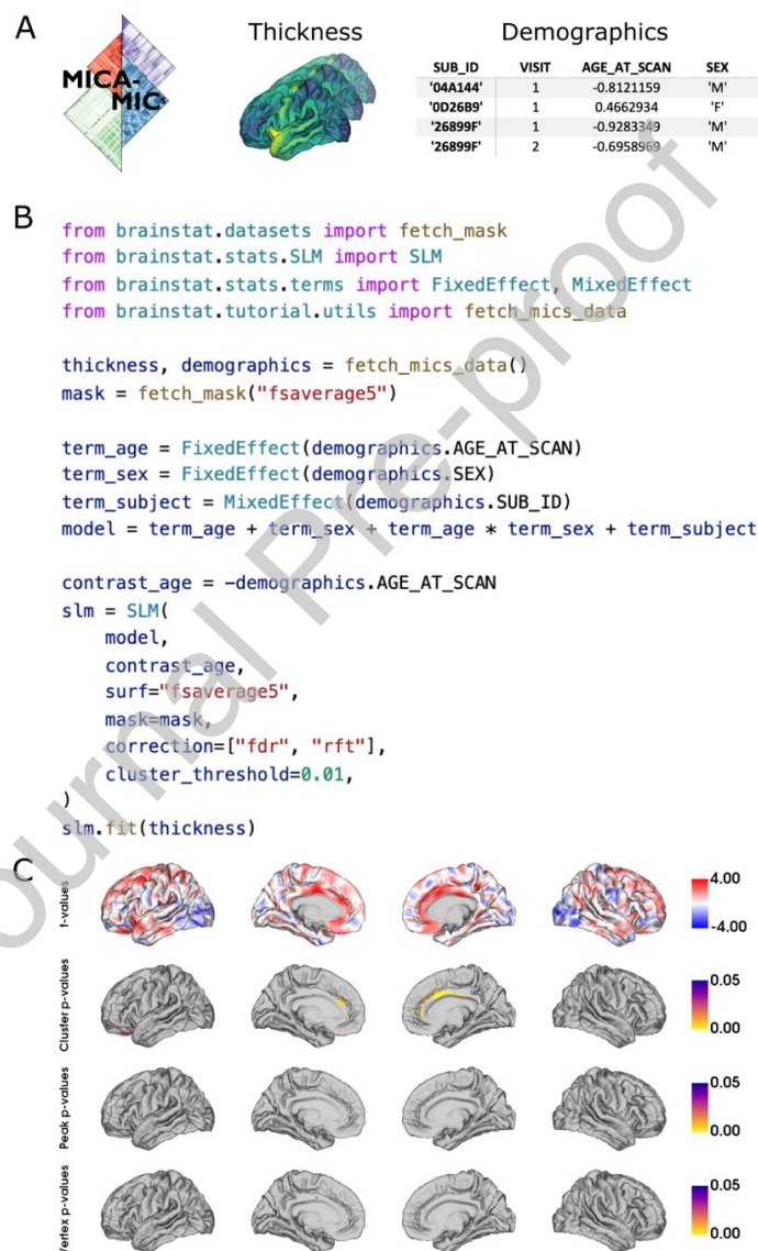
Figure 2. Example Python code for fitting a fixed effect general linear model of the effect of age on cortical thickness with BrainStat. (A) The MICA-MICS data included with
