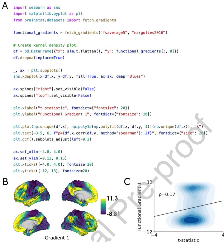
Figure 4. Association to functional gradients. (A) Example Python code for computing and plotting the correlation of the t-statistic map and the first functional gradient. Cortical surface plotting code was omitted for brevity. See the supplemental Jupyter notebook (Python) and live script (MATLAB) for executable versions of this code as well as additional figure building code. (B) First functional gradient plotted onto the brain surface. (C) Kernel density plot of the t-statistic map and the first functional gradient.
