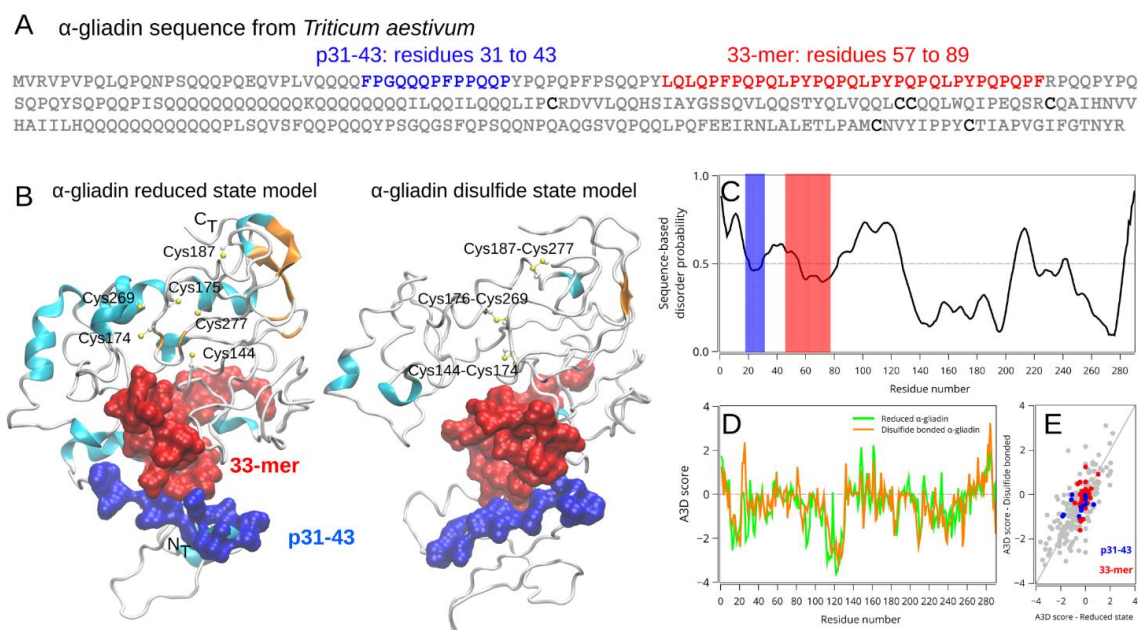
Figure 2. Structural characterization of the reduced and oxidized states of \alpha -2-gliadin of Triticum aestivum . Primary sequence of wheat \alpha -2-gliadin where the p31-43 (blue) and 33-mer (red) regions are highlighted (A). Tridimensional structure of \alpha -2-gliadin in the obtained previously [19] and the new disulfide state model (B). The immunogenic regions are in surface representation using the same color reference as in panels A and C, and the cysteine pairs involved in disulfide bonds are marked for clarity. Sequence disorder prediction was calculated using the PrDOS server (C), and the aggregation propensity was calculated using AGGRESCAN 3D (D) for both oxidation states. The horizontal gray line in panel C marks the 5% threshold (false positive rate), while aggregation-prone regions have positive values, respectively. The per residue correlation between both oxidation states is shown in panel (E).
