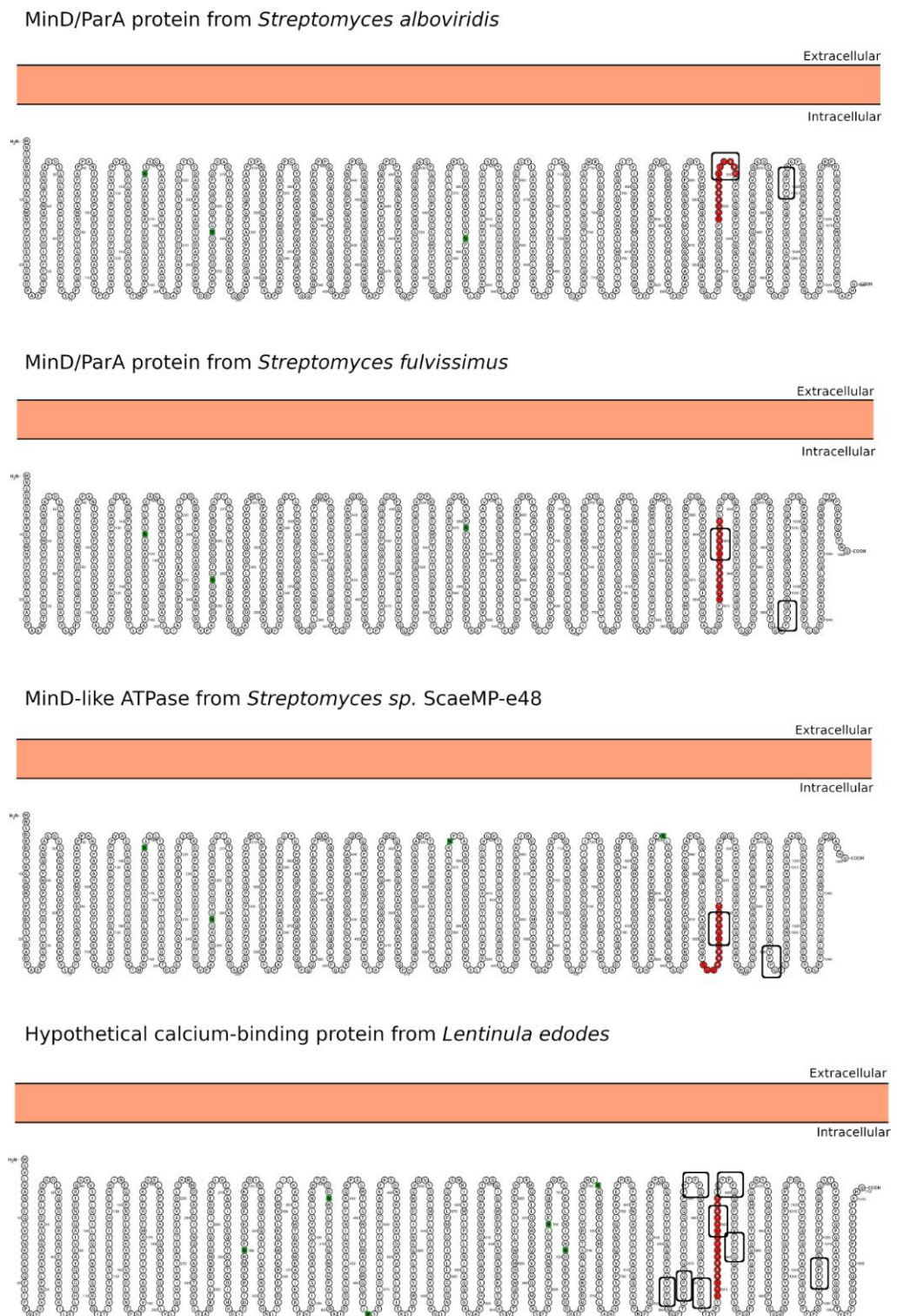
Figure 7. Predicted subcellular localization for the BLASTp hits proteins using the p31-43 sequence as a query. The localization of the high similarity sequence regions from the four best BLASTp hits is shown in red. The Y/FPPQ-binding motif recognized by the WW domain is highlighted with a rectangle. The analysis was performed using the Protter server [82]. The N-glycosylation motifs are marked as green squares.
