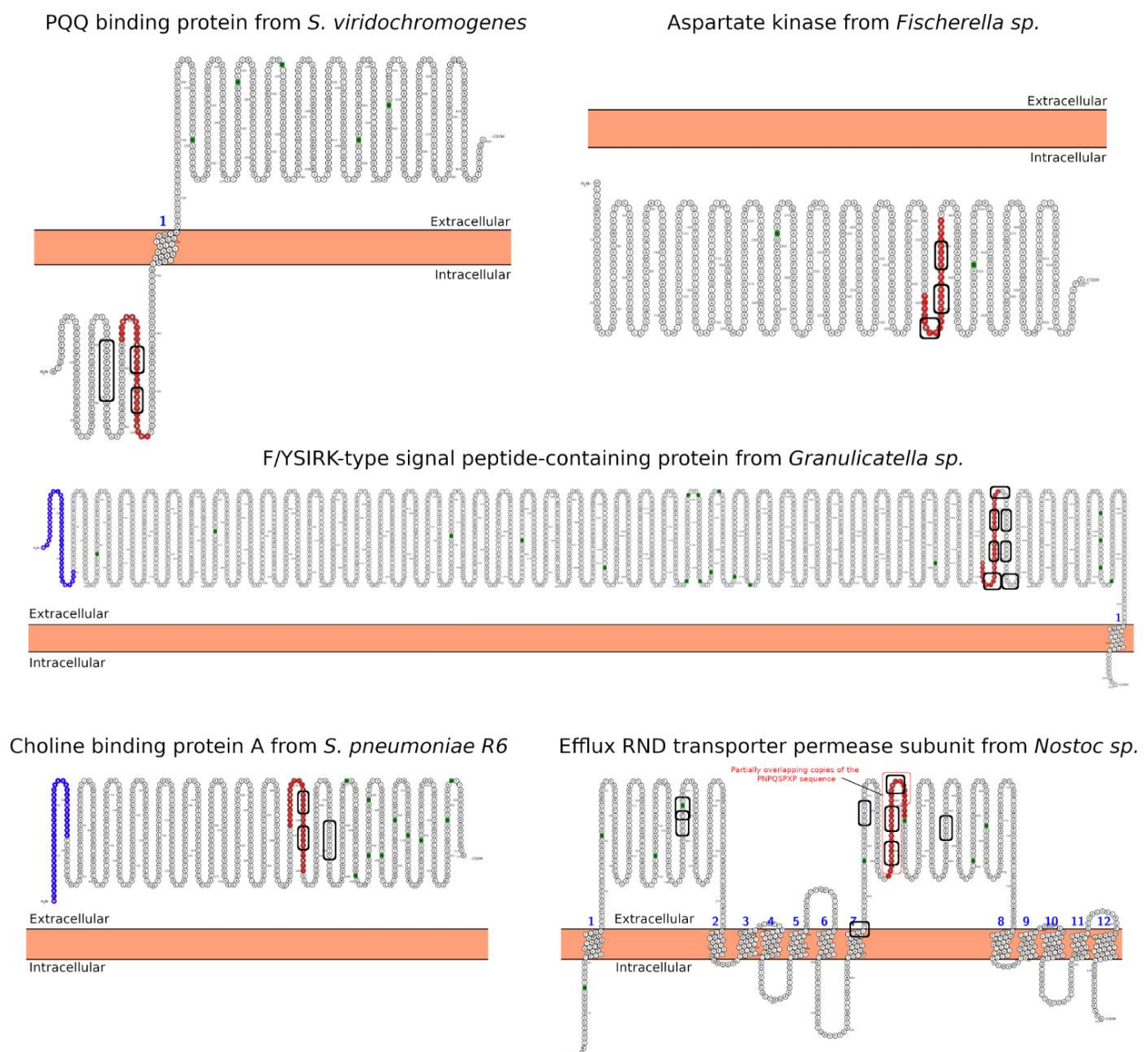
Figure 6. Predicted subcellular localization for the BLASTp hits proteins using the 33-mer sequence as query. The localization of the high similarity sequence regions from the five best BLASTp hits is shown in red. The SH3-binding motifs are highlighted with a rectangle. The analysis was performed using the Protter server [82]. The partially overlapping copies of the PNPQSPXP sequence in the RND efflux pump protein are shown as a red rectangle. The signal peptides are shown in blue and N-glycosylation motifs are marked as green squares.
