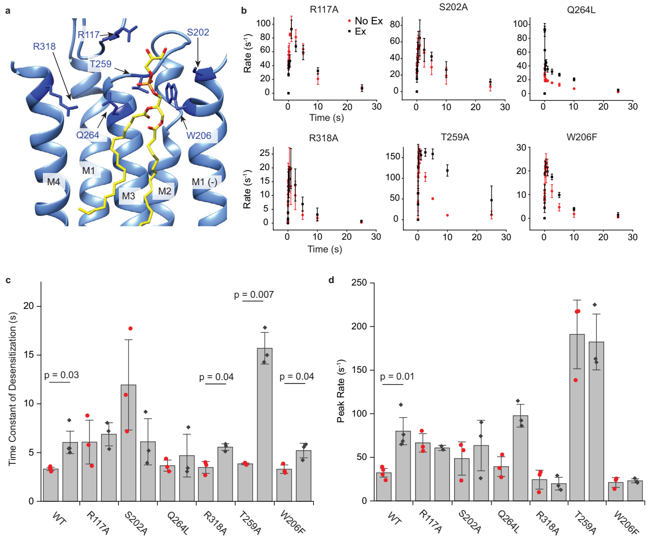
Fig. 6 | Mutational analysis of the outer leaflet phospholipid binding site. a ELIC5 CA structure showing POPG (yellow) at the outer leaflet site and residues (dark blue) targeted by mutagenesis. b TI + flux rates of mutants in response to 10 mM propylamine for no-exchange (red) and exchange (black, 25 mol% POPG in the outer leaflet) conditions ( n = 3 ). Source data are provided as a source data file. c Weighted time constant of desensitization in response to 10 mM propylamine for
