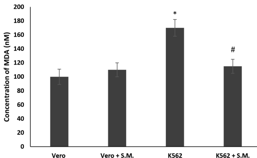
Figure 3. Lipid peroxidation inhibitory activity in K562 cells and Vero cells treated with Skeletonema marinoi (S.M.) for 48 h at a concentration of 0.75 mg/mL. Data are expressed by the means \pm standard deviation (SD) of three experiments. (* p < 0.05 means a significant difference between the Vero and K562 cells; # p < 0.05 means a significant difference between the treated and untreated K562 cells).
