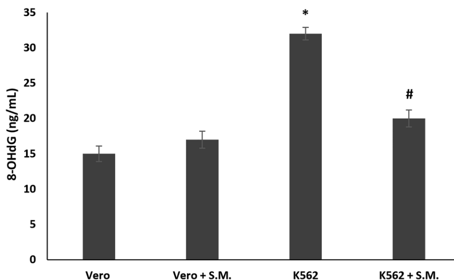
Figure 6. Effects of Skeletonema marinoi (S.M.) (0.75 mg/mL) on oxidative DNA damage of K562 and Vero cells after 48 h of treatment. Data were represented by the means \pm standard deviation (SD) of three experiments. (* p < 0.05 means a significant difference between the Vero and K562 cells; # p < 0.05 means a significant difference between the treated and untreated K562 cells).
