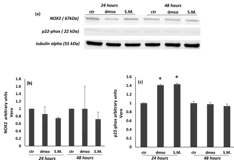
Figure 9. Effect of Skeletonema marinoi (S.M.) on NOX2 and p22-phox protein levels in Vero cells after 24 and 48 h of treatment. Panel (a): representative Western blot of NOX 2 and p22-phox in Vero cells; panel (b): densitometric analysis of NOX2; panel (c): densitometric analysis of p22-phox. Experiments were conducted in triplicates, and the values were normalized towards the tubulin. Densitometric analyses were expressed as arbitrary units. Data are shown as mean \pm standard deviation (SD) and were compared by ANOVA (* p < 0.05 versus untreated Vero cells).
