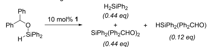
Scheme 5. The catalytic hydrosilylation of benzophenone with \mathbf{1} with \text{D}_2\text{SiPh}_2 ( \text{R} = \text{H/D} or \text{OC(H/D)Ph}_2 ) (top). The H/D exchange of \mathbf{1} to \mathbf{1D} with a deuterated silane (middle). The siloxane scrambling catalyzed by \mathbf{1} (bottom).
