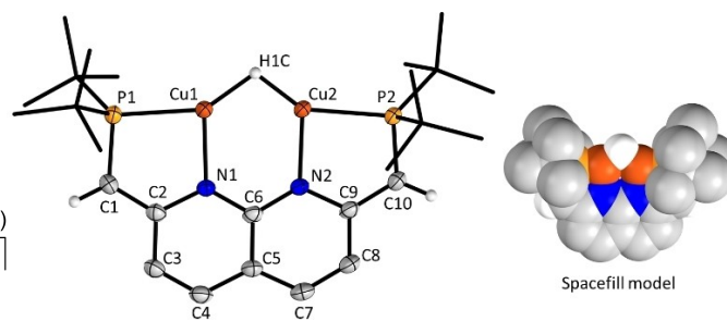
Figure 1. The structure of 1 determined by X-ray diffraction. Displacement ellipsoids (left) are displayed at 50% probability, t-Bu groups are depicted as wireframe, and the K (18-crown-6) counterion and two THF molecules are omitted for clarity. Spacefill spheres (right) are shown at the Van der Waals radius.
