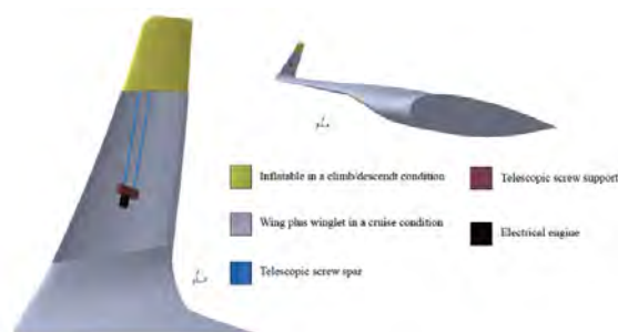
Figure 1: Telescopic device concept
