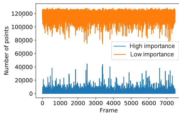
FIGURE 4. Number of points in high- and low-importance regions.
