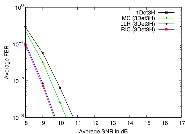
FIGURE 5. Average FER performance versus average SNR \bar{\gamma} of MC, LLR, RIC over frequency-selective fading channel. The number of helper MSs h is three. No quantization is applied for the LLR scheme.
