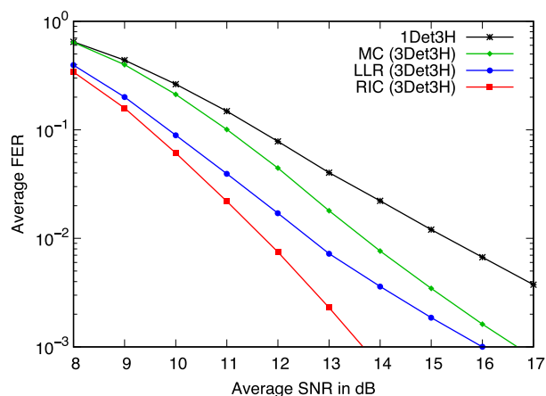
FIGURE 4. Average FER performance versus average SNR \bar{\gamma} of MC, LLR, RIC over the frequency-flat fading channel. The number of helper MSs h is three. No quantization is applied for the LLR scheme.
