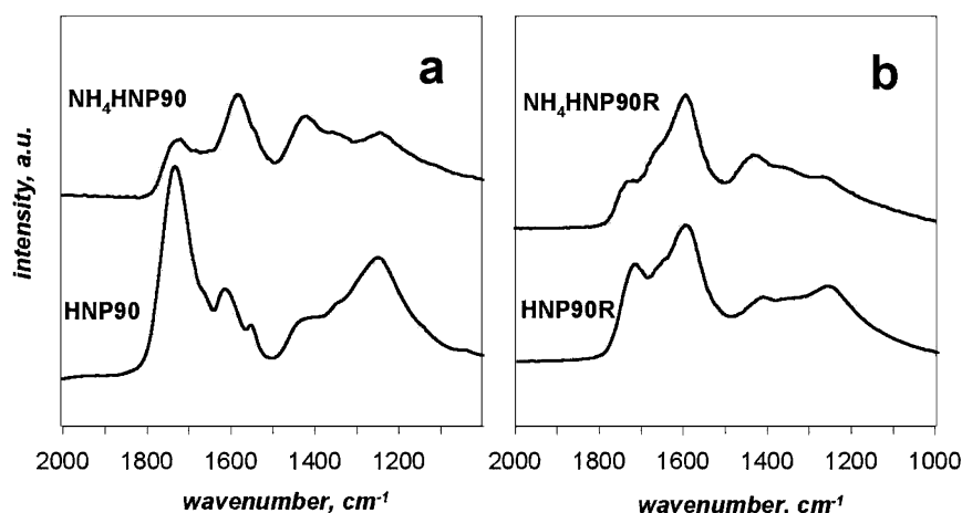
Figure 2. ATR-FTIR spectra of (a) HNP90 and (b) HNP90R together with the corresponding ammonium salt in the 1000–2000 \text{cm}^{-1} region.
