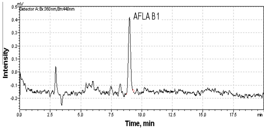
Fig. 2. Fluorescence chromatogram of a AFB 1 standard at 1 µg/kg.
