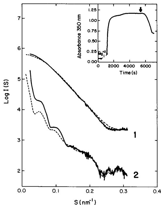
FIGURE 8 X-ray scattering traces of 80 \mu\text{M} GDP-tubulin-taxol in PEDTA, 1 mM GDP at 37°C before ( curve 1 ) and 120 to 370 s after ( curve 2 ; final pH 6.7) the addition of 7 mM \text{MgCl}_2 . The dashed line 1 is the dimer scattering model 1 (Fig. 3). The dashed line 2 corresponds to 35% single linear oligomer and 65% microtubule models (Fig. 3). ( Inset ) Turbidity time course (47.5 \mu\text{M} GDP-tubulin-taxol)
