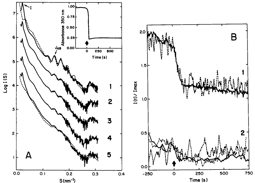
FIGURE 6 Effect of temperature on the self-association of 85 \mu\text{M} GDP-tubulin in PEDTA, 1 mM GDP, 7 mM \text{MgCl}_2 (pH 6.7). (A) Curve 1, solid line, x-ray scattering profile at 2°C (the dashed line 1 is the ring scattering model 1 from Fig. 1); curves 2–5, average profiles after a temperature shift to 37°C; curve 2, second 0 to 250; curve 3, second 500 to 750; curve 4, second 750 to 1000; curve 5, second 1400 to 2000; the dashed line 5 corresponds to 80% model single linear oligomers and 20% model double rings (from models 4 and 1, respectively, in Fig. 1). (Inset) Time course of turbidity (60 \mu\text{M} GDP-tubulin). (B) Solid line 1, time course of the intensity of the ring interference peak I during the experiment in A; dashed line 1, time course of the ring J_{05} -like Bessel function peak; lines 2, time course of intensity of the central scattering and of the scattering vector intervals that would correspond to the J_{02} and J_{12} microtubule signals (see Fig. 7).
