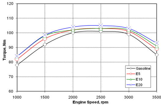
Fig1.3. Brake torque versus engine speed, at 25% full throttle
