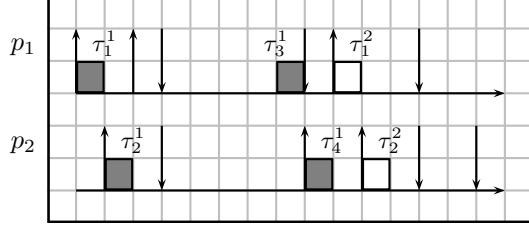
Figure 6: The example of Figure 5 scheduled by DDSP.
