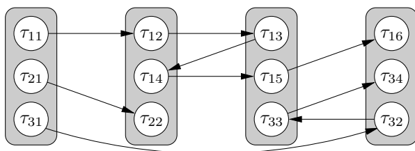
Figure 1: An example of 3 pipelines over 4 processors.
