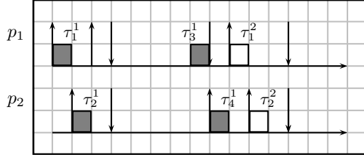
Figure 5: Counterexample for the simple protocol.
