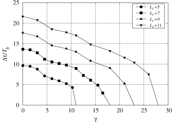
Fig. 10. Contour curves corresponding to an E_b/N_0 penalty of -3 dB for a \text{BER} = 10^{-12} , versus \Delta\tau/T_b and \gamma . QPSK modulation is considered.
