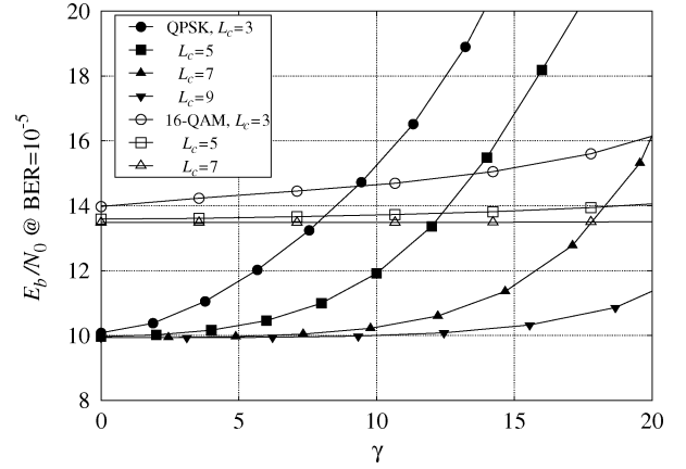
Fig. 8. Values of E_b/N_0 necessary to obtain a BER of 10^{-5} versus the value of \gamma , when only GVD is present.
