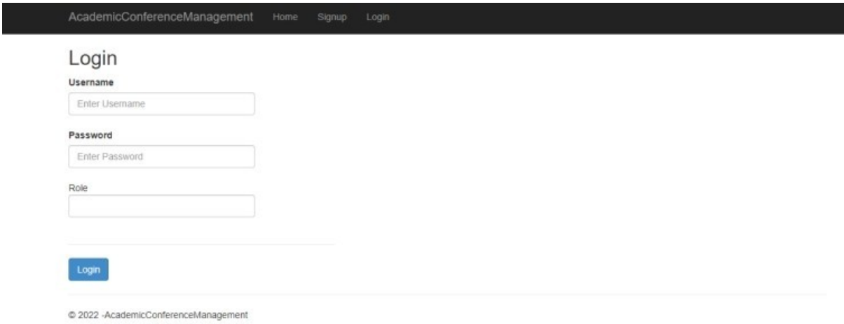
Figure 11: Login Interface
