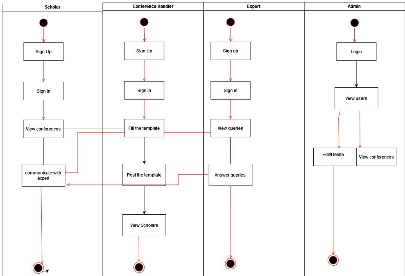
Figure 2: Application flow
