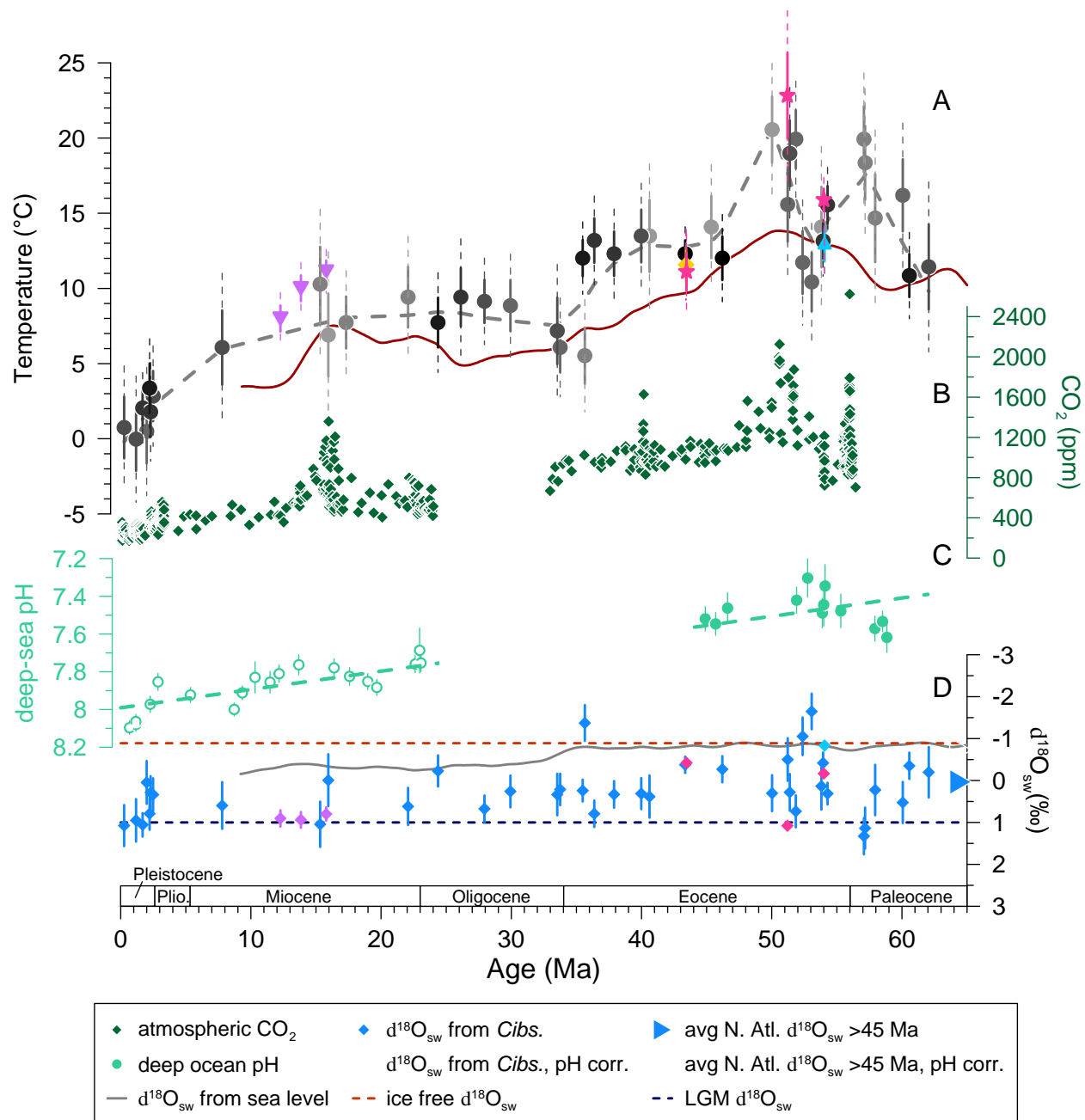
5 Fig. 2. Cenozoic evolution of seawater isotopic composition and comparison with changes in the carbon cycle. (A) \Delta_{47} temperatures as in Fig. 1 with (B) atmospheric CO 2 concentration from boron isotopes in planktic foraminifera (Rae et al., 2021) with 1 SD uncertainties, and (C) reconstructed deep ocean pH from boron isotopes in benthic foraminifera ((Greenop et al., 2017),
