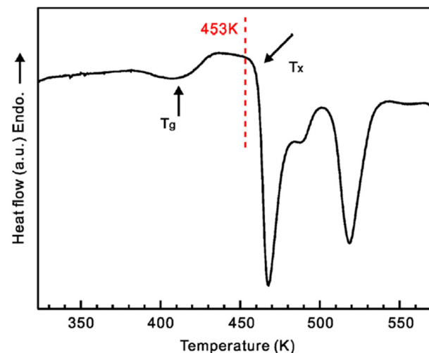
Figure 7. Differential scanning calorimetry scan for the \text{Mg}_{65}\text{Cu}_{20}\text{Zn}_5\text{Y}_{10} metallic glass. Reprinted from [58], Copyright (2014), with permission from Elsevier.
