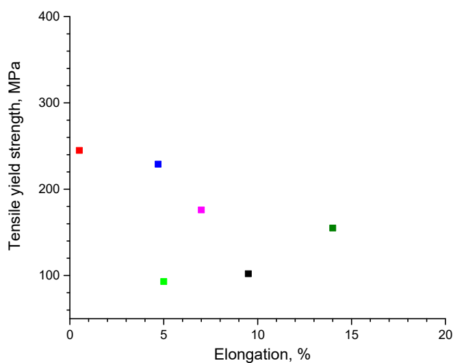
Figure 18. Tensile yield strength–elongation data for Al and Al alloy matrix composites: ■ Al + Ni 60 Nb 40 [55]; ■ Al-Zn-Ca + Co 48 Cr 15 Mo 14 C 15 B 6 Tm 2 [73]; ■, ■ Al 2024 + Fe 49.9 Co 35.1 Nb 7.7 B 4.5 Si 2.8 [57]; ■ Al + Al 84 Gd 6 Ni 7 Co 3 [56]; ■ Al + Zr 48 Cu 36 Ag 8 Al 8 [69].
