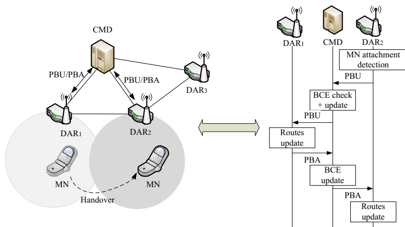
Fig. 4 Partially distributed network-based HDMM: CMD behaves as PBU/PBA relay.
