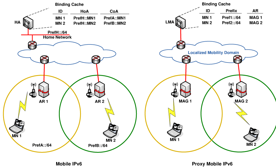
Fig. 1 Centralized IP mobility protocols operation.
