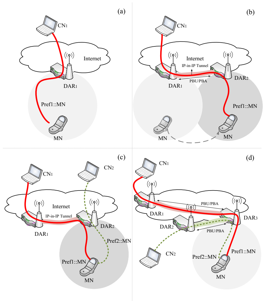
Fig. 8 Fully distributed network-based HDMM: protocol operation.
