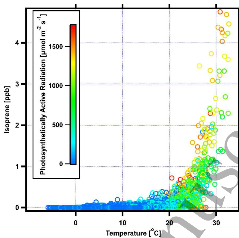
Figure 1. Hourly isoprene mixing ratios measured by GC-MS at the Auchencorth Moss site between 2008 and 2014 as a function of ambient air temperature, with individual points coloured by photosynthetically active radiation.
