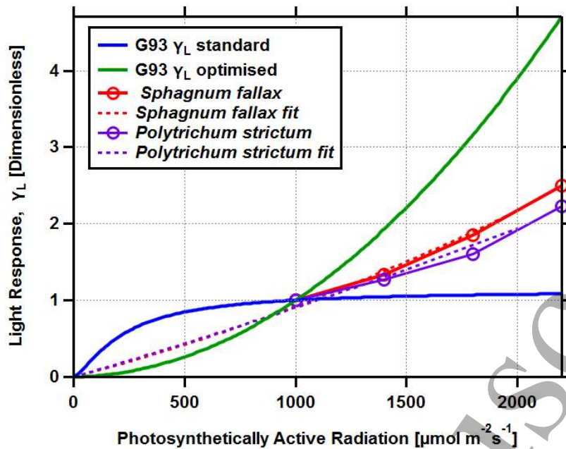
Figure 3. Whole-plant isoprene light response curves for the mosses Sphagnum fallax (red) and Polytrichum strictum (purple) when measured in spring (solid) relative to the classical Guenther (G93) light response curve (blue) and the optimised light response curve (green) that best describes the ecosystem-level eddy covariance flux measurements at the Auchencorth Moss site. Dashed lines show an extrapolation of the Sphagnum fallax and Polytrichum strictum light response curves based on a 3-point quadratic fit to the observations.
