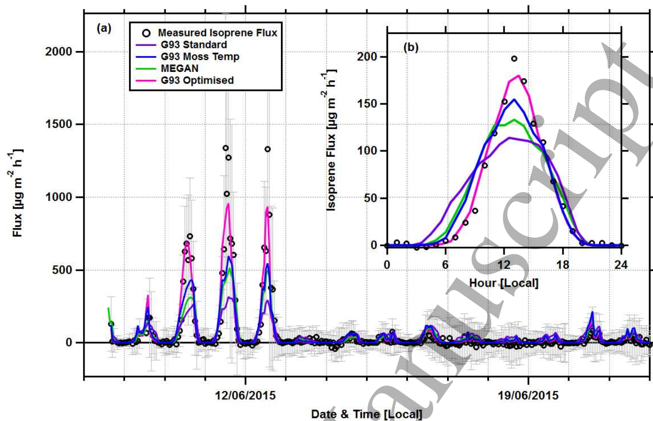
Figure 5. Hourly measured isoprene fluxes measured at the Auchencorth Moss field site (black circles) plotted alongside isoprene emissions predicted by the MEGAN model (green) and G93 emission algorithms, with both standard (purple) and optimised (pink) light response curves. Error bars represent the random error associated with individual flux measurements (see SI). Inset Panel b shows the average diurnal cycle of the four traces. The isoprene emission potentials used for each algorithm were (G93 Standard = 769 \mu\text{g m}^{-2} \text{h}^{-1} , G93 Moss Temp = 146 \mu\text{g m}^{-2} \text{h}^{-1} , G93 Optimised = 1,039 \mu\text{g m}^{-2} \text{h}^{-1} , MEGAN = 1,930 \mu\text{g m}^{-2} \text{h}^{-1} )
