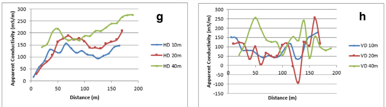
Fig. 3. Terrain conductivity plot along traverses 1-4 on dumpsite (HD and VD).
