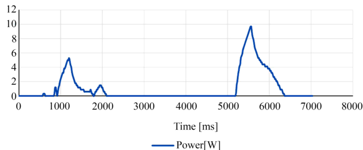
Fig. 10. Power consumption test results [W] for a ripe tomato
