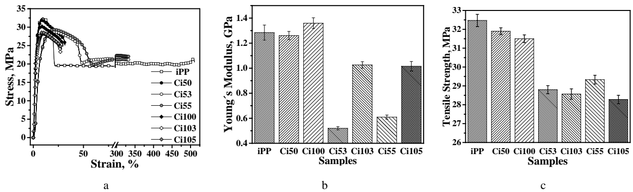
Fig. 3. Tensile test results of pure iPP and Ci50, Ci53, Ci55, Ci100, Ci103, and Ci105 composites: a–stress-strain curves of all samples; b–Young's modulus; c–tensile strength
