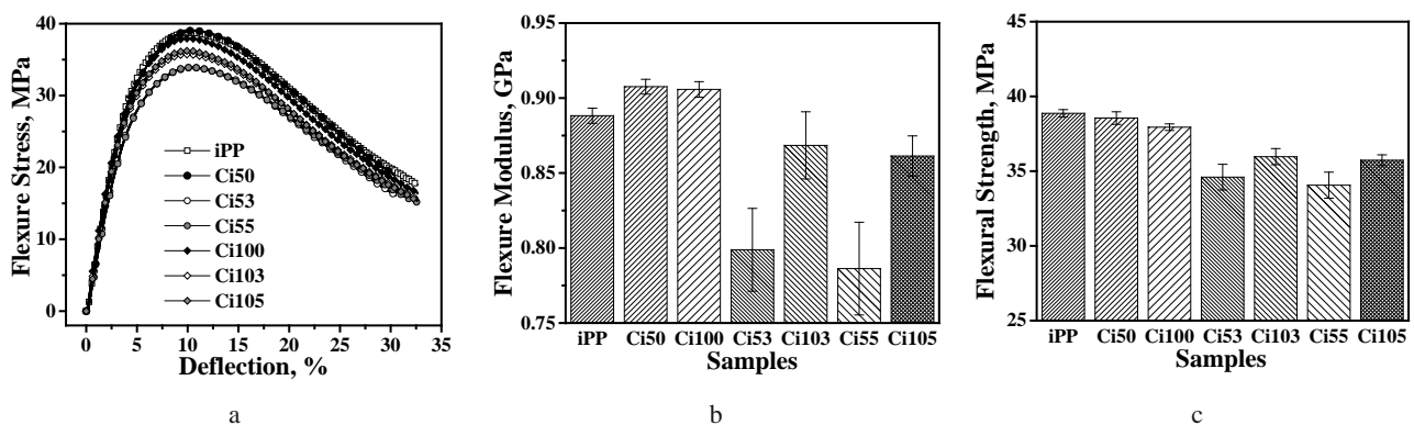
Fig. 4. Flexural test of pure iPP and Ci50, Ci53, Ci55, Ci100, Ci103, and Ci105 composites to room temperature: a–flexure stress-deflection; b–flexure modulus; c–flexural strength
