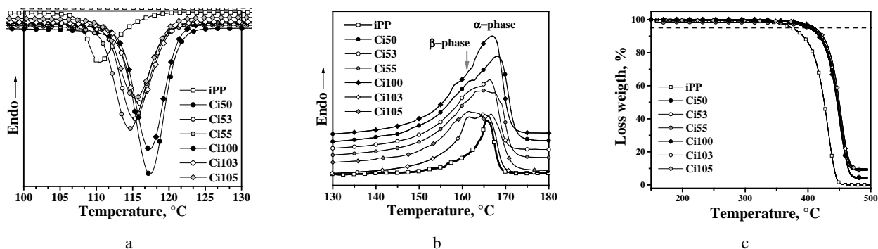
Fig. 10. DSC analysis: a – crystallization; b – melting curves; c – TGA analysis for pure iPP and composites
