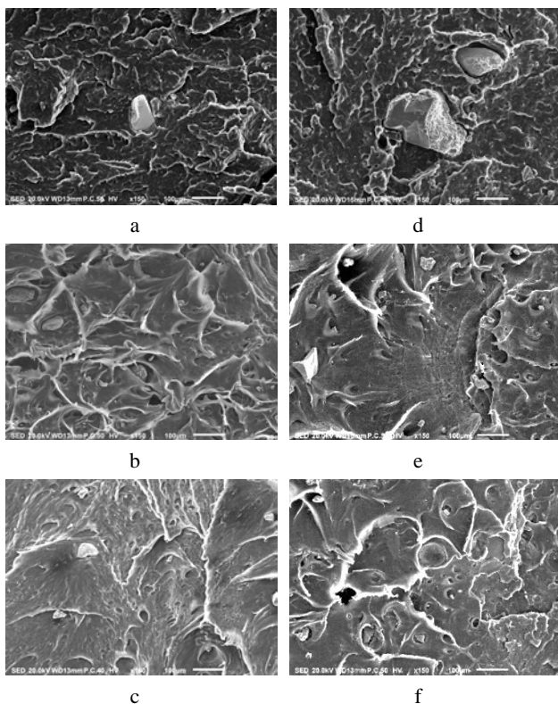
Fig. 7. SEM images cryogenic fractured composites after flexural test: a–Ci50; b–Ci53; c–Ci55; d–Ci100; e–Ci103; f–Ci105 composites
