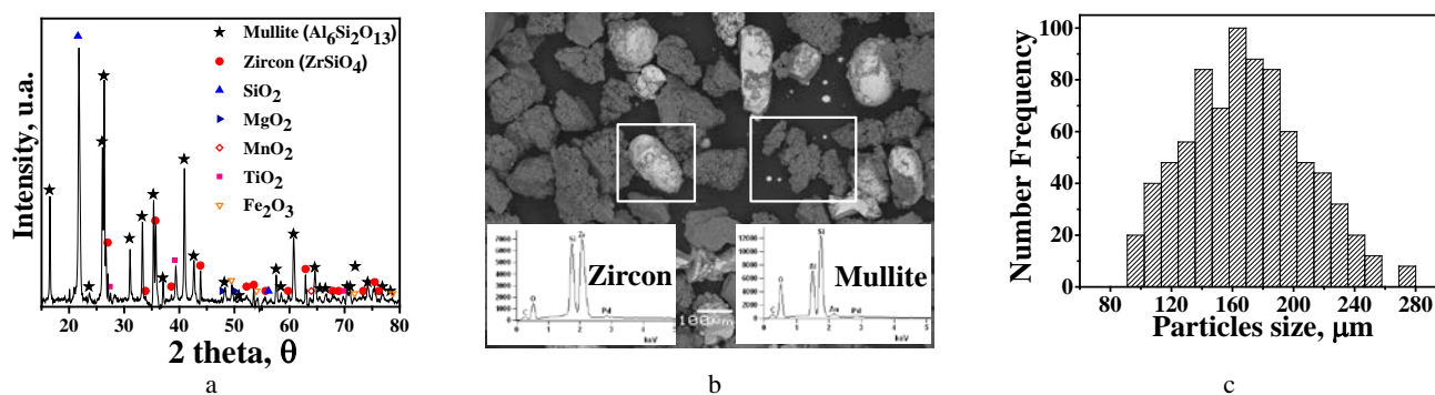
Fig. 1. a – DRX pattern of ceramic waste; b – SEM morphology and EDS elemental analysis of CW; c – particle sizes distribution of CW
