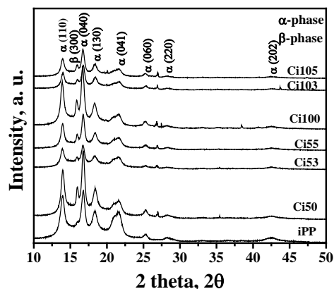
Fig. 8. XRD pattern of pure iPP and composites
