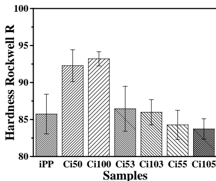
Fig. 5. Hardness test of pure iPP and composites
