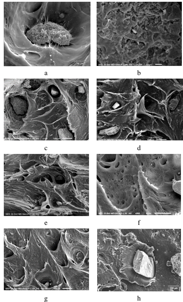
Fig. 6. SEM images fracture surface composites after tensile test: a, e—interfacial interaction by mechanical adhesion composites; b—Ci50; c—Ci53; d—Ci55; f—Ci100; g—Ci103; h—Ci105 composites
