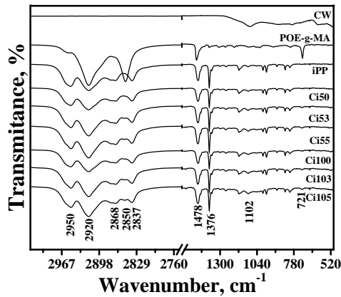
Fig. 9. FTIR spectra of pure iPP and composites
