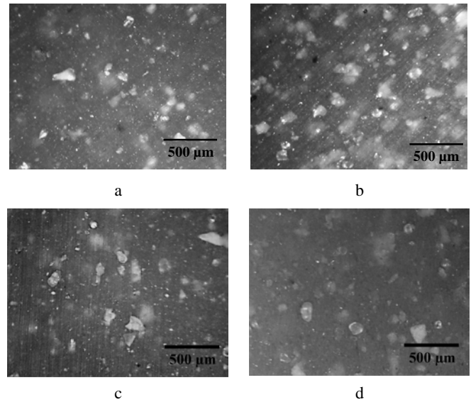
Fig. 2. OM images of composite: a–Ci50; b–Ci100; c–Ci55; d–Ci105 with 5 wt.% of POE-gMAH, both
