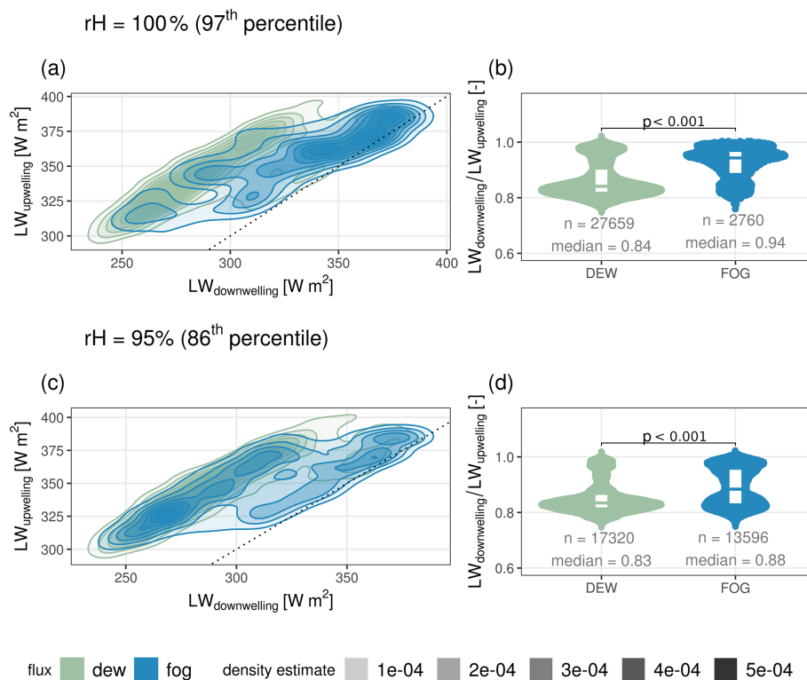
Figure G3. Comparison of upwelling LW and downwelling LW during the conditions classified as having fog and dew from the flux partitioning of the lysimeter weight changes based on a rH threshold of 100% (a, b) and 95% (c, d). Panels (a) and (c) illustrate the smoothed kernel density estimate, with the black dotted line displaying the identity line. Panels (b) and (d) illustrate the distribution of radiation ratios during dew and fog conditions. The differences between the distributions are statistically significant, with a significance level p < 0.001 .
