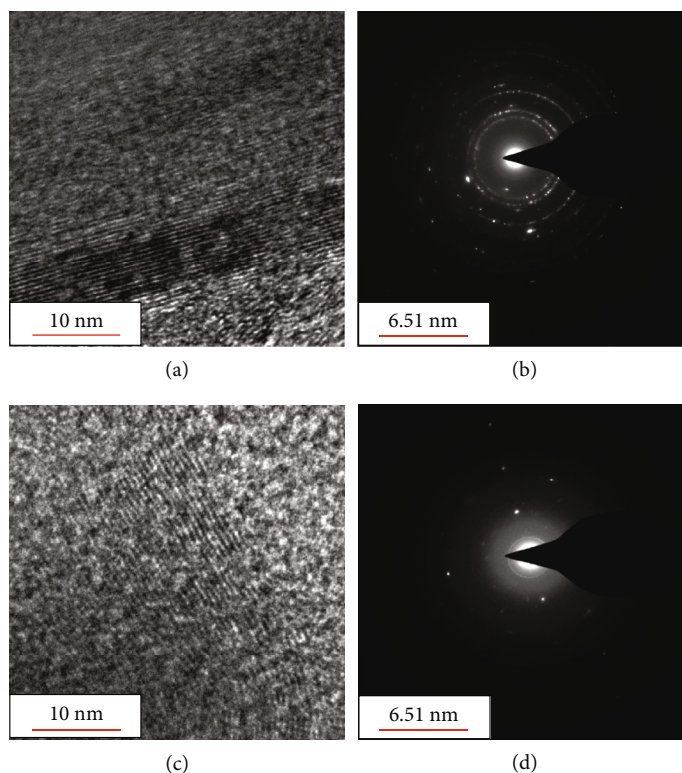
FIGURE 3: The TEM images and diffraction images of deep shales at different maturity evolution stages. (a) TEM image of sample 5, (b) diffraction image of sample 5, (c) TEM image of sample 8, and (d) diffraction image of sample 8.
