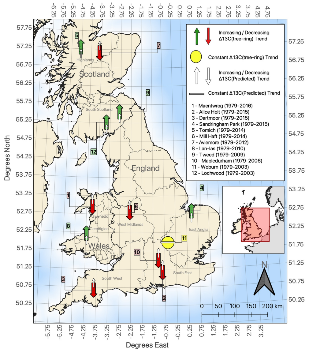
Figure 4. Predicted and tree-ring based trends in \Delta^{13}C over the period 1979–2016 at each site.
